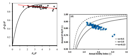
Figure 1 Plots of the annual (P-Q)/P data in the HRC (left, this study) and in the NLRB (right, Istanbuluoglu et al., 2012)
