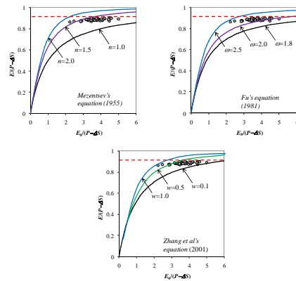
Figure 1 Plots of the annual water balance at the HRC, China, in the modified Budyko space (dots) and the Budyko curves determined with different formulas. The red dashed line indicates the possible bounded ET in the water limited condition.
