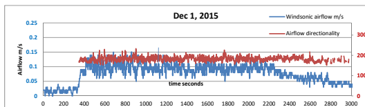
Figure 3. The airflow (blue) is seen to be clockwise ( 180^\circ ) red) during the period of cooling and beyond, as the airflow falls away after 35 minutes. That observation fits in with the net air density between the two columns at each period prior to and following the switching on and off of the refrigeration.
