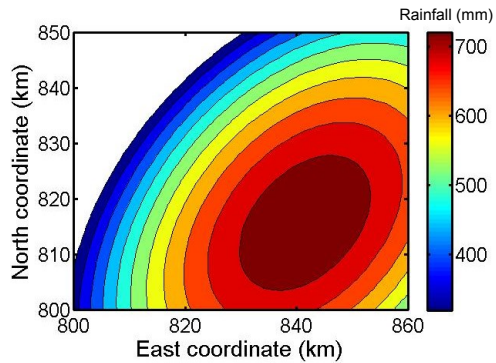
Fig. 18. 24-hour PMP with NE-SW orientation 45^\circ centered at Hong Kong Island
