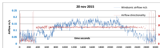
Figure 1. Number 1 experiment of 20 November, 2015. With the 150 Watt halogen lamp switched on, the directionality prior to condensation is counter-flow. Abrupt change at around 320 s when the refrigeration is switched on and again after 35 minutes.
