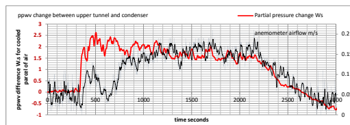
Figure 3. Left hand Y-axis show the ppwv change rate in W.s. The right hand Y-axis is the observed airflow, for the experiment of 20 November, 2015.
