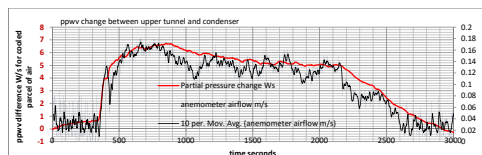
Figure 3. Experiment 19 Nov, 2015, as above. The profile of the condensation partial pressure change at the cooling coils fits the airflow curve remarkably well. That indicates that the counter flow as seen in Figure 2, with air flowing from the left hand column to the right hand column is overcome.
