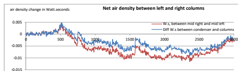
Figure 2. Similar pattern as in other experiments with right hand column heating. The counter-clockwise flow is apparent, taking into account the cool air from the condenser (blue). The peak at around 500 s corresponds with a rise in the airflow.
