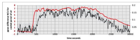
Figure 3. Second experiment of 20 November, 2015. Again we observe a good 'fit' between the observed airflow and the partial pressure change from condensation.
