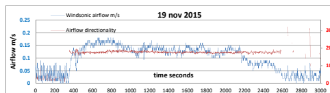
Figure 1. Experiment 19 Nov, 2105, with 100 Watt lamp heating air right hand column. The directionality of airflow changes abruptly at approx 330 s, when the refrigeration is switched on. It does so again at 2150 s when the refrigeration is switched off.
