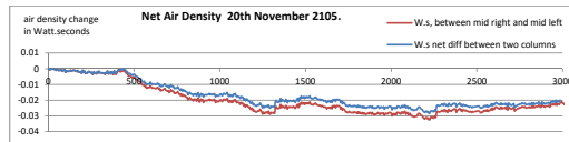
Figure 2. The same pattern as during experiment of 19 November, with the net kinetic energy of the two columns indicating counter-clockwise flow. At around 440 s the net kinetic energy flow indicates a peak when the flow has briefly become clockwise. That coincides with the 'blip' in the observed airflow in its transition from counter-clockwise to clockwise flow. The difference between the two curves shows the impact of including the cold, dense air generated at the cooling coils.
