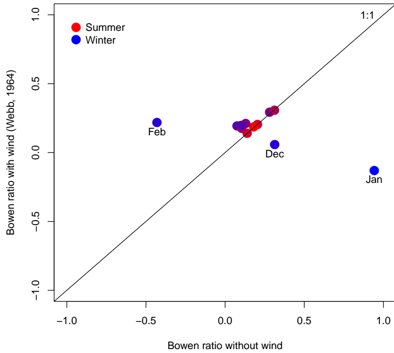
Fig. 1. Comparing Bowen ratio
