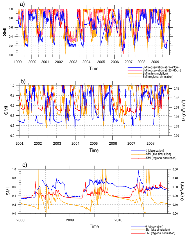
Figure 2. Soil moisture dynamics at the three micrometeorological sites: (a) Hyytiälä, (b) Sodankylä and (c) Kenttäröva, comparing results from regional (the model grid boxes where the sites are located) and site JSBACH simulations with observations. The volumetric soil moisture ( \theta ) is shown for the Sodankylä and Kenttäröva sites.
