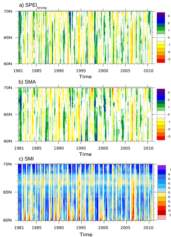
Figure 4. Latitude–time transections of (a) SPEI forcing , (b) SMA and (c) SMI over Finland in the study period (the summer months (June, July, August) in 1981–2010).
