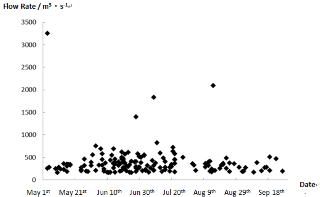
Fig. 1. scatter plot of flood occurrence time based on POT method
