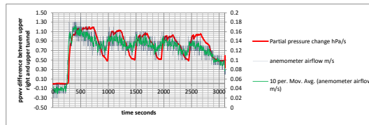
Figure 2 Airflow versus condensation. Experiment March 3, 2015
