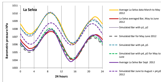
Figure 1. Barometric tidal wave, La Selva, Costa Rica
