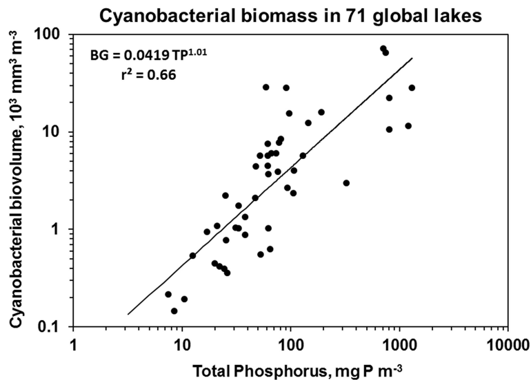
Fig. 1. Relationship between summer mean concentrations of cyanobacterial biovolume and total phosphorus in 71 lakes located worldwide. Data from Smith (1985) and V.H. Smith (unpubl.)
