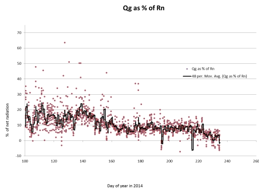
Figure 1 - Measured soil heat flux ( Q_g/G ) as percentage of Net radiation ( R_n ) during daytime: 10 to 16h over the course of the growing season.
