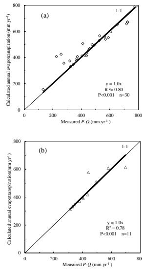
Figure 8. Scatter plots of calculated evapotranspiration using equation (7 & 8) against E_s = P-Q during calibration phase (a) and validation period (b). The thin line is the 1:1 line and the bold line is the line of best-fit provided by the equation.
