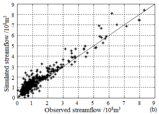
Fig. 8. Comparison of observed and modelled monthly streamflow in 1971-2010 (a)TOPMODEL (b) VIC model
