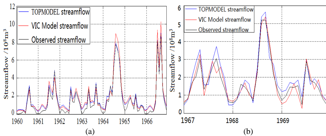
Fig.6. the simulated and observed streamflow for the calibration and validation period for TOPMODEL and VIC model (a) calibration period (b) validation period
