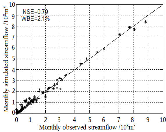
(a) calibration streamflow for TOPMODEL
