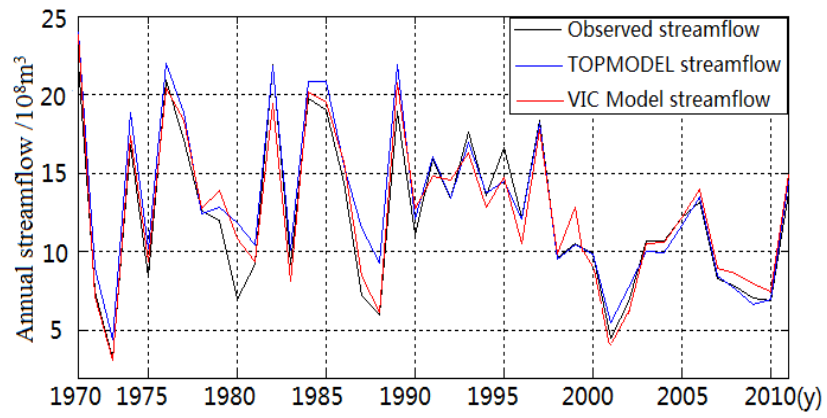
Fig. 9. Time series of observed and model simulated annual streamflow for JRB for the entire modelling period
