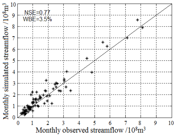
(c) calibration streamflow for VIC model
