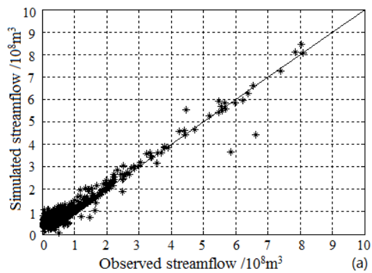
Fig. 8. Comparison of observed and modelled monthly streamflow in 1971-2010 (a)TOPMODEL (b) VIC model
