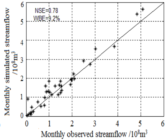
(b) validation streamflow for TOPMODEL
