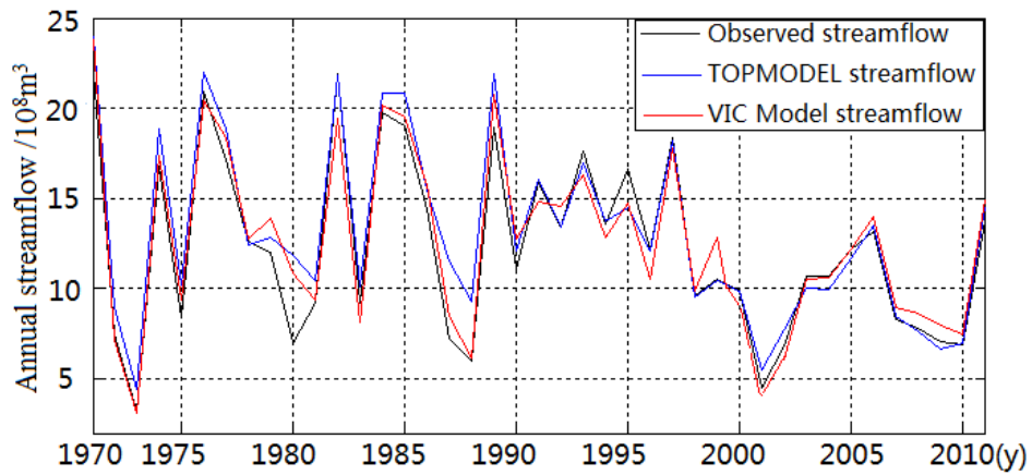
Fig. 9. Time series of observed and model simulated annual streamflow for JRB for the entire modelling period
