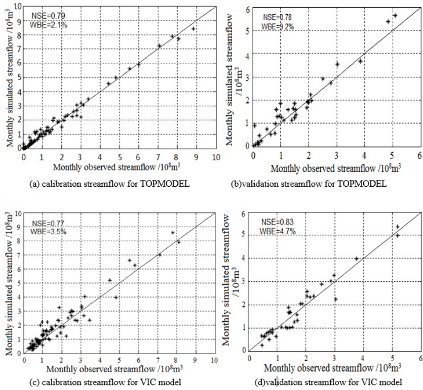
Fig. 7. Comparison of observed and modelled monthly streamflow for calibration and validation periods
