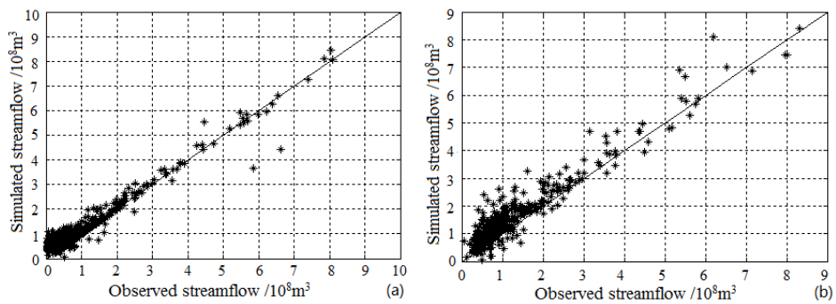
Fig. 8. Comparison of observed and modelled monthly streamflow in 1971-2010 (a)TOPMODEL (b) VIC model
