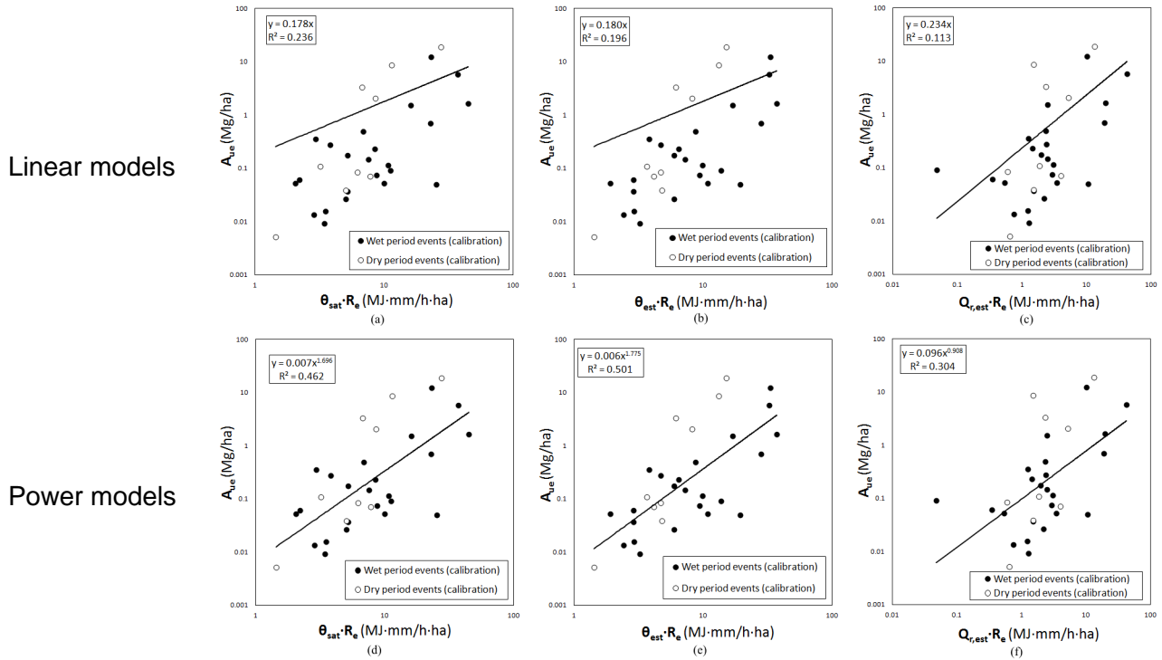
Figure 3. Regression models between measured soil loss A_{Ue} and the erosivity indices \theta \cdot R_e and Q \cdot R_e for the calibration dataset. Linear models (a), (b), (c): SM4E model and satellite soil moisture (a); SM4E model and estimated soil moisture (b); USLE-M model and estimated runoff coefficient (c). Power models (d), (e), (f): SM4E model and satellite soil moisture (d); SM4E model and estimated soil moisture (e); USLE-MM model and estimated runoff coefficient (f).
