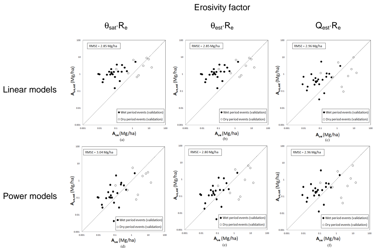
Figure 4. Testing of the A_{ue} vs \theta \cdot R_e and the A_{ue} vs Q \cdot R_e models for the validation dataset: Linear models (a), (b), (c): SM4E model and satellite soil moisture (a); SM4E model and estimated soil moisture (b); USLE-M model and estimated runoff coefficient (c). Power models (d), (e), (f): SM4E model and satellite soil moisture (d); SM4E model and estimated soil moisture (e); USLE-MM model and estimated runoff coefficient (f).
