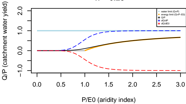
Turc–Mezentsev formula n= 6.25
