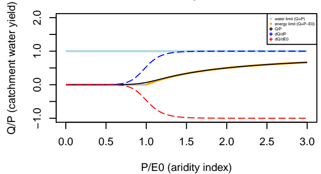
Tixeront–Fu formula n= 10.44
