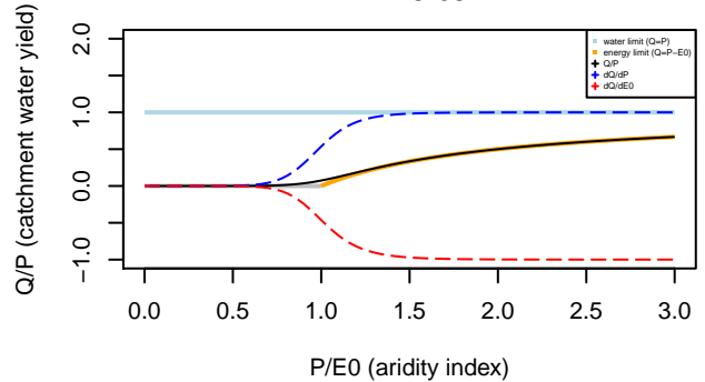
Tixeront–Fu formula n= 9.69
