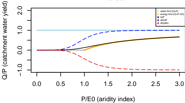
Turc–Mezentsev formula n= 5.00
