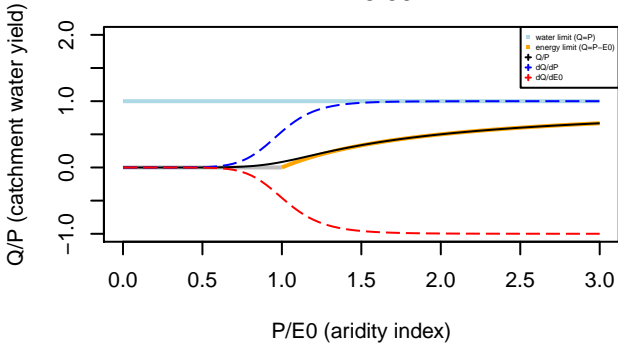
Turc–Mezentsev formula n= 8.00
