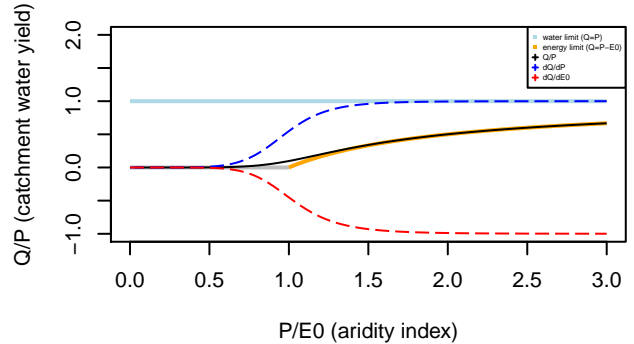
Tixeront–Fu formula n= 7.44
