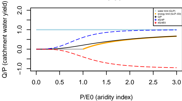
Turc–Mezentsev formula n= 3.00
