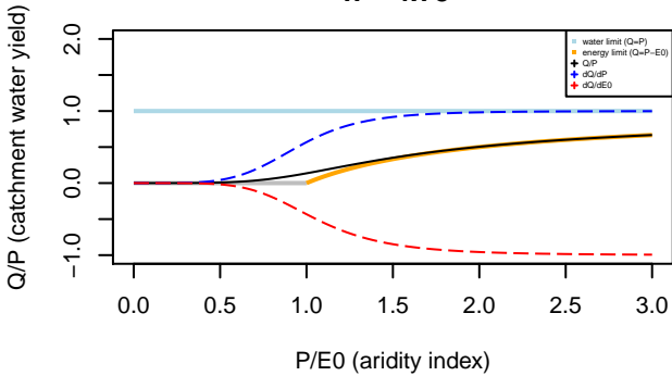
Turc–Mezentsev formula n= 4.75
