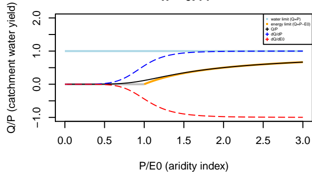
Tixeront–Fu formula n= 6.44
