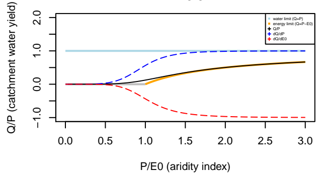
Tixeront–Fu formula n= 5.94
