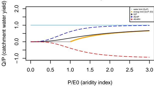
Turc–Mezentsev formula n= 2.75
