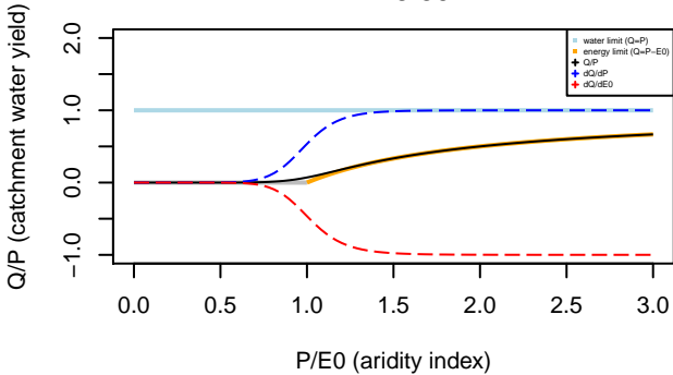
Turc–Mezentsev formula n= 9.50
