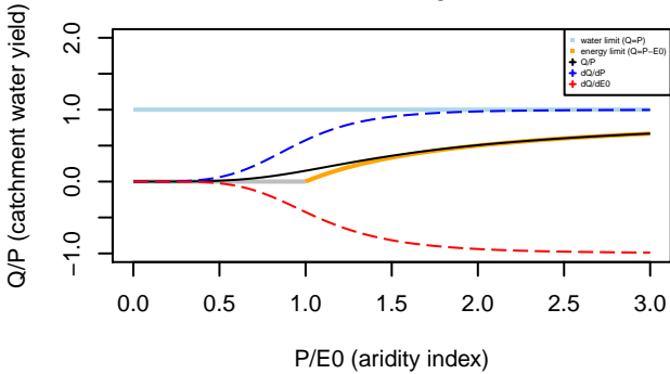
Turc–Mezentsev formula n= 4.25
