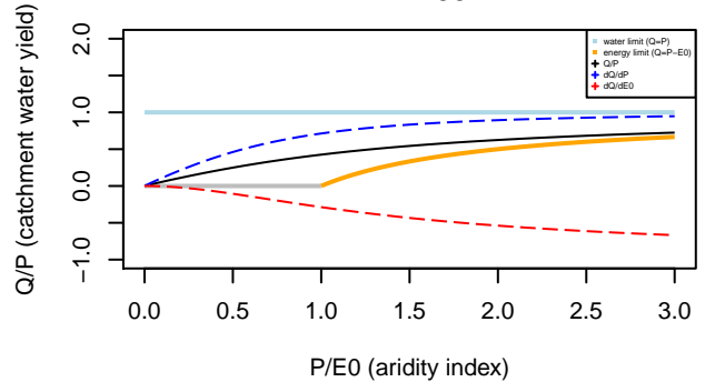
Tixeront–Fu formula n= 1.95
