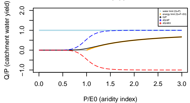
Tixeront–Fu formula n= 8.69
