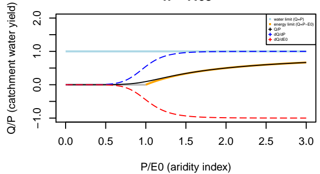
Tixeront–Fu formula n= 7.69
