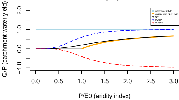
Turc–Mezentsev formula n= 3.25
