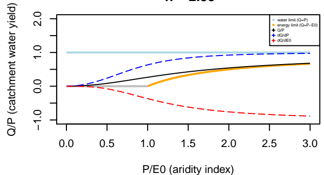
Tixeront–Fu formula n= 2.95
