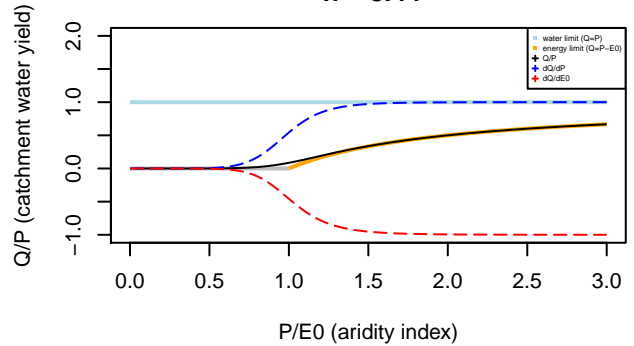
Tixeront–Fu formula n= 8.44
