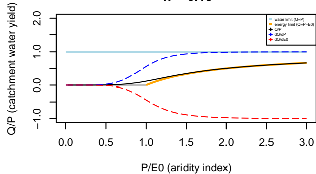
Tixeront–Fu formula n= 6.19
