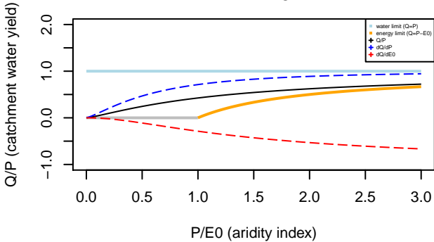
Turc–Mezentsev formula n= 1.25
