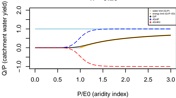
Turc–Mezentsev formula n= 9.25
