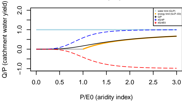
Turc–Mezentsev formula n= 3.75
