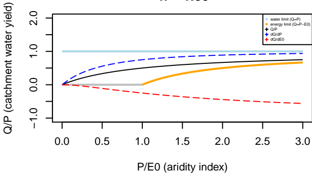
Turc–Mezentsev formula n= 1.00
