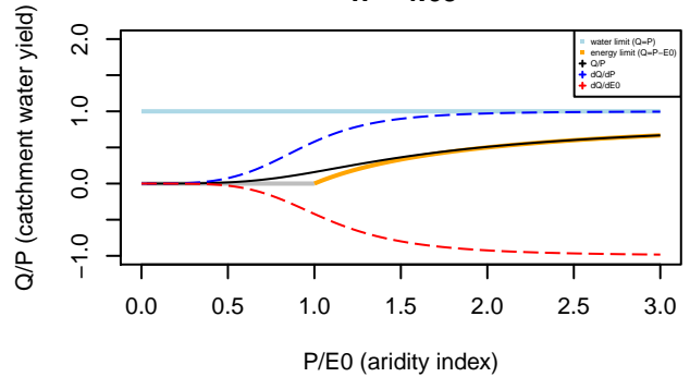
Tixeront–Fu formula n= 4.69
