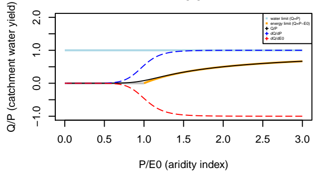
Tixeront–Fu formula n= 8.94
