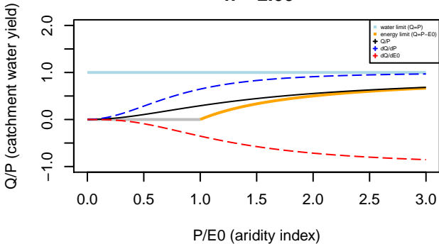
Turc–Mezentsev formula n= 2.00
