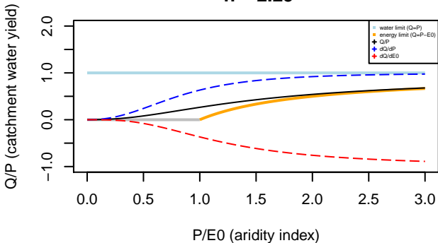
Turc–Mezentsev formula n= 2.25
