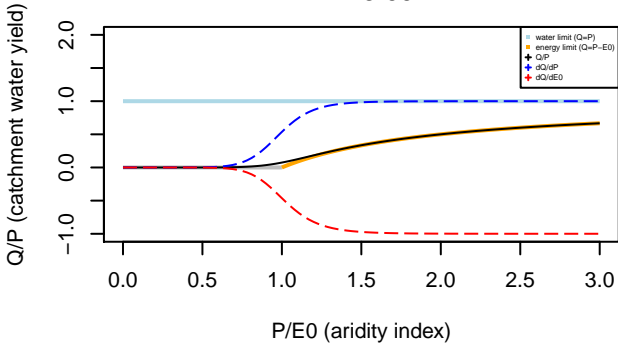
Turc–Mezentsev formula n= 9.00
