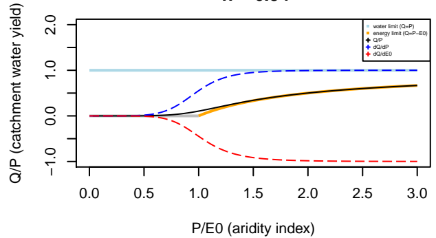
Tixeront–Fu formula n= 6.94
