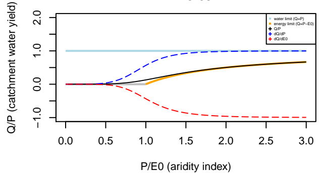
Tixeront–Fu formula n= 5.69
