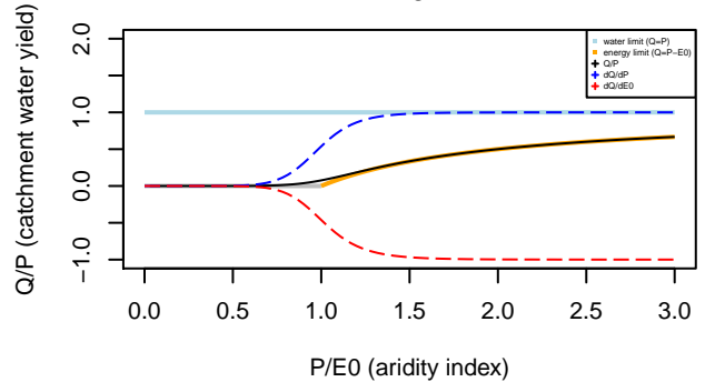
Tixeront–Fu formula n= 9.44
