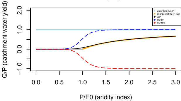
Turc–Mezentsev formula n= 8.75
