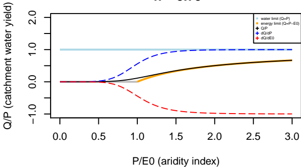
Turc–Mezentsev formula n= 5.75
