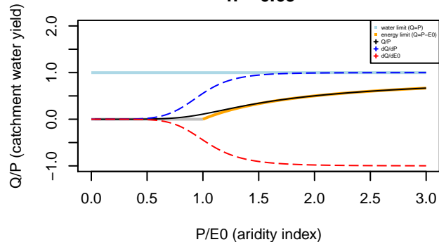
Tixeront–Fu formula n= 6.69
