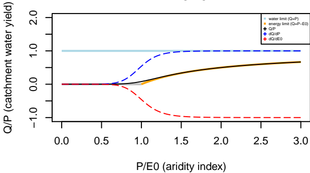
Turc–Mezentsev formula n= 8.25
