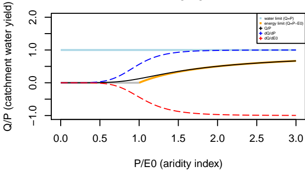
Turc–Mezentsev formula n= 5.25
