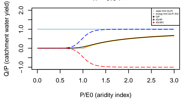
Tixeront–Fu formula n= 9.94
