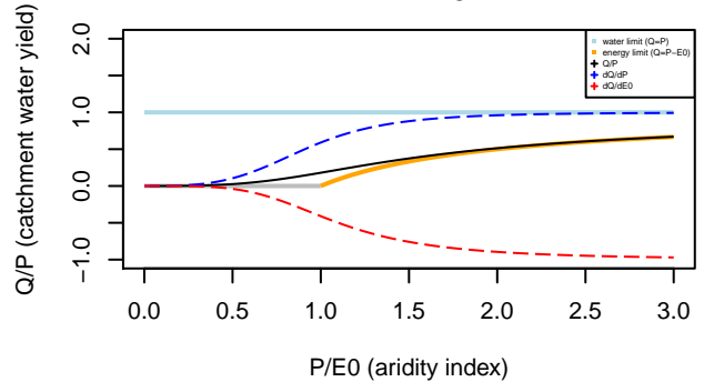
Tixeront–Fu formula n= 4.20
