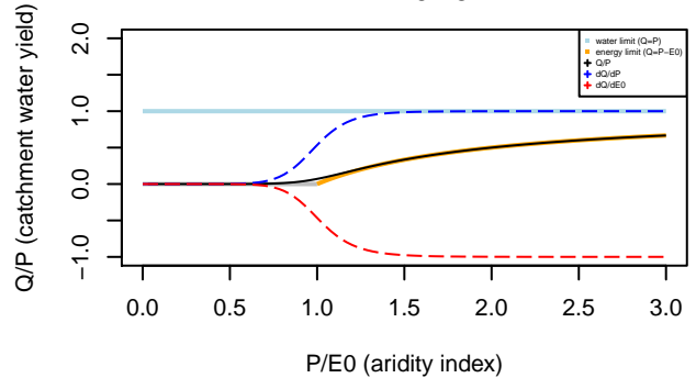
Tixeront–Fu formula n= 10.19
