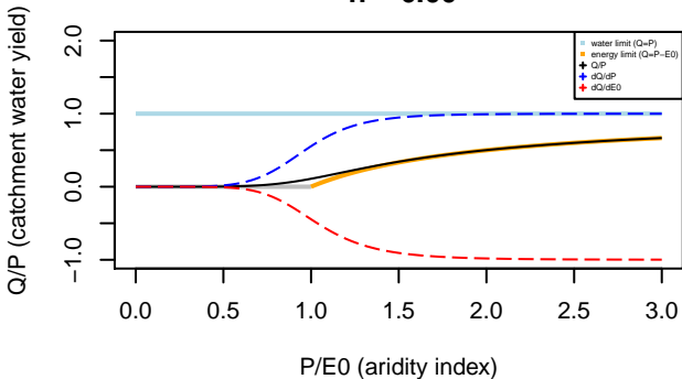
Turc–Mezentsev formula n= 6.00
