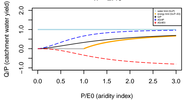
Tixeront–Fu formula n= 2.45
