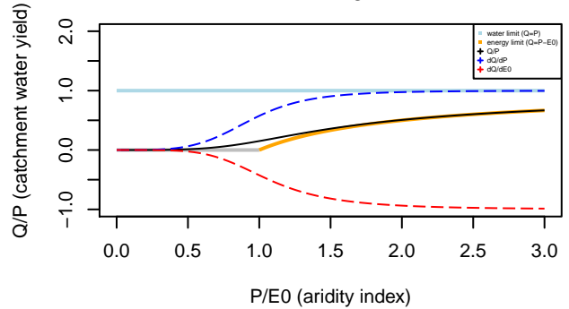
Tixeront–Fu formula n= 4.94
