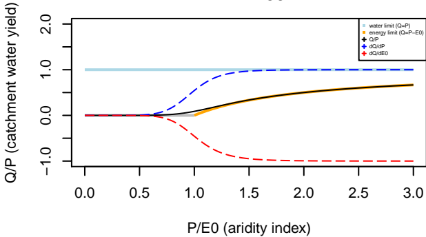
Turc–Mezentsev formula n= 7.50
