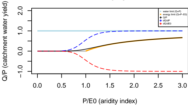
Turc–Mezentsev formula n= 6.75
