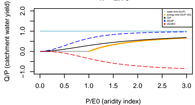
Tixeront–Fu formula n= 2.70
