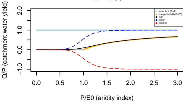
Turc–Mezentsev formula n= 7.00
