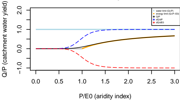
Turc–Mezentsev formula n= 7.25
