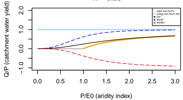
Tixeront–Fu formula n= 3.20
