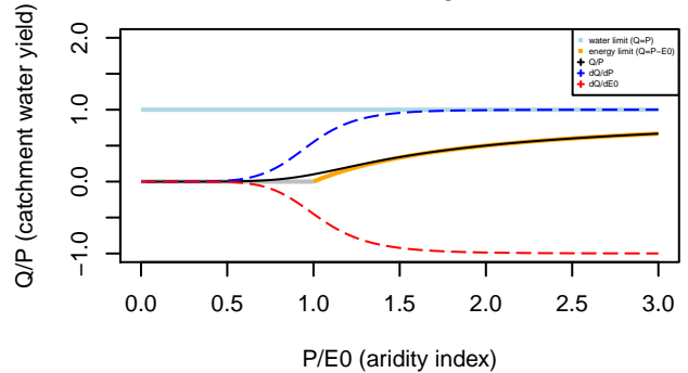
Tixeront–Fu formula n= 7.19
