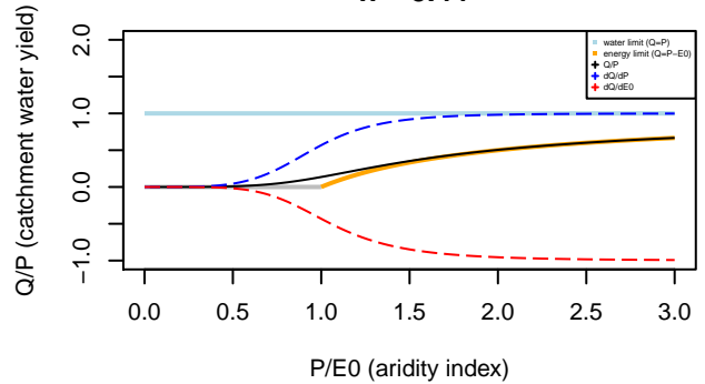
Tixeront–Fu formula n= 5.44
