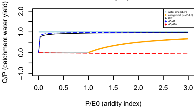
Turc–Mezentsev formula n= 0.25
