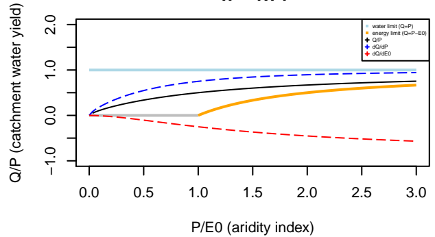
Tixeront–Fu formula n= 1.71
