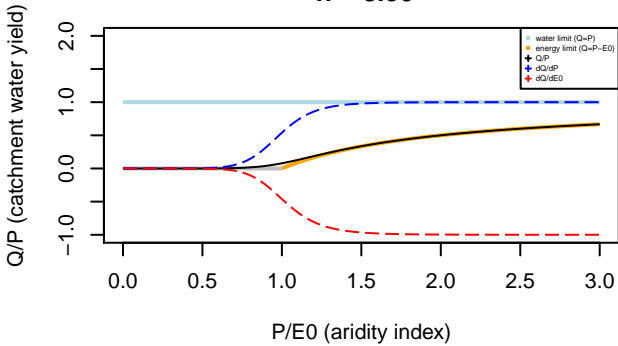
Turc–Mezentsev formula n= 8.50
