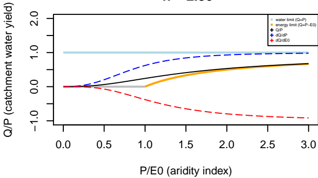
Turc–Mezentsev formula n= 2.50
