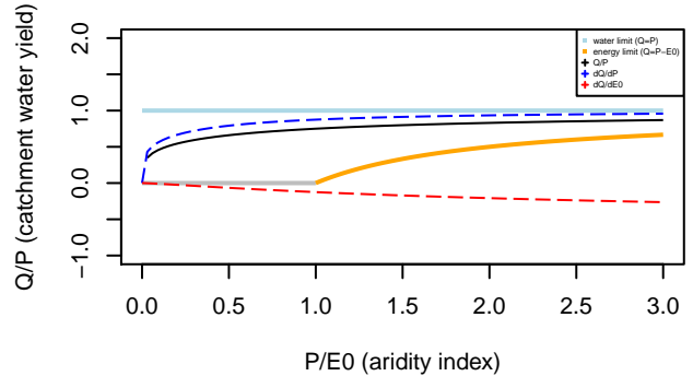
Tixeront–Fu formula n= 1.24
