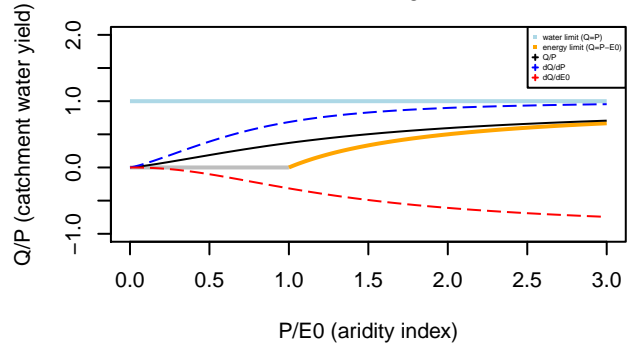
Tixeront–Fu formula n= 2.20
