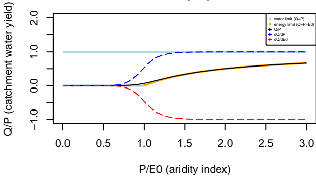
Turc–Mezentsev formula n= 9.75
