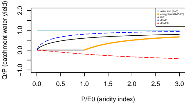
Turc–Mezentsev formula n= 0.75
