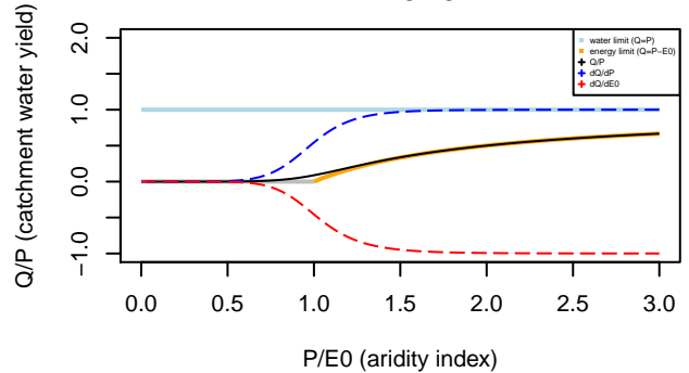
Tixeront–Fu formula n= 8.19
