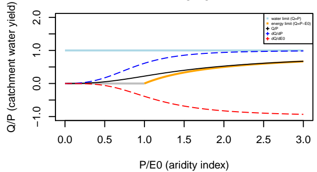
Tixeront–Fu formula n= 3.45
