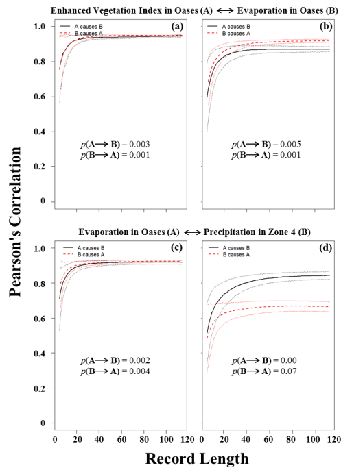
Fig. 5. Convergence Cross Mapping
