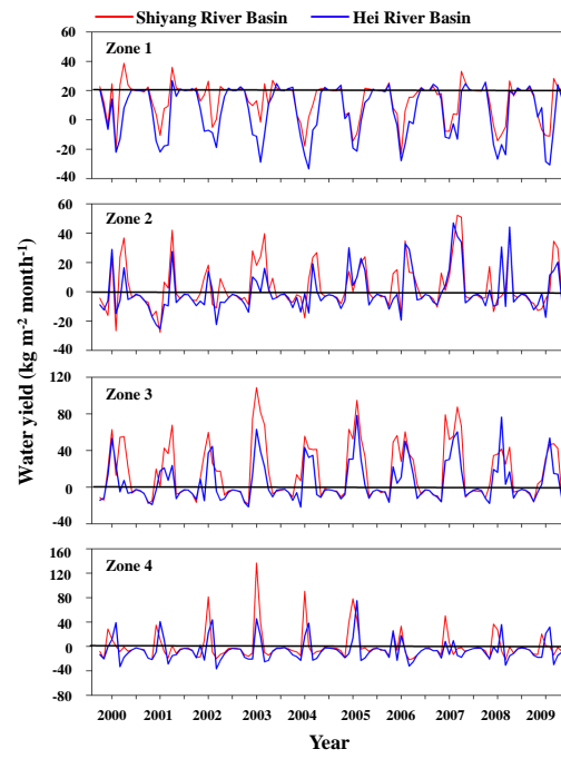
Fig. 9. Within-zone water yields
