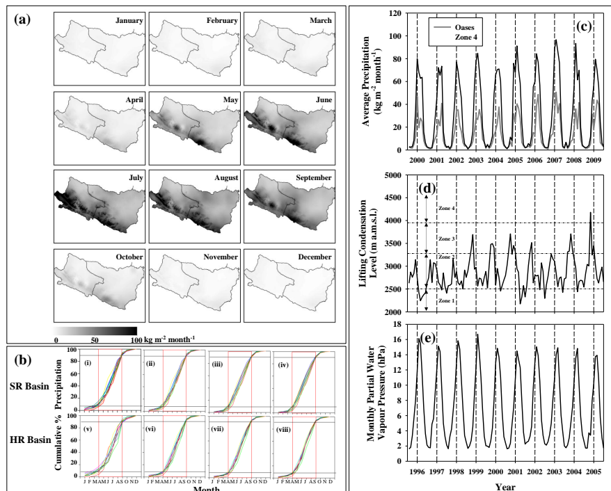
Fig. 6. Precipitation and associated variables
