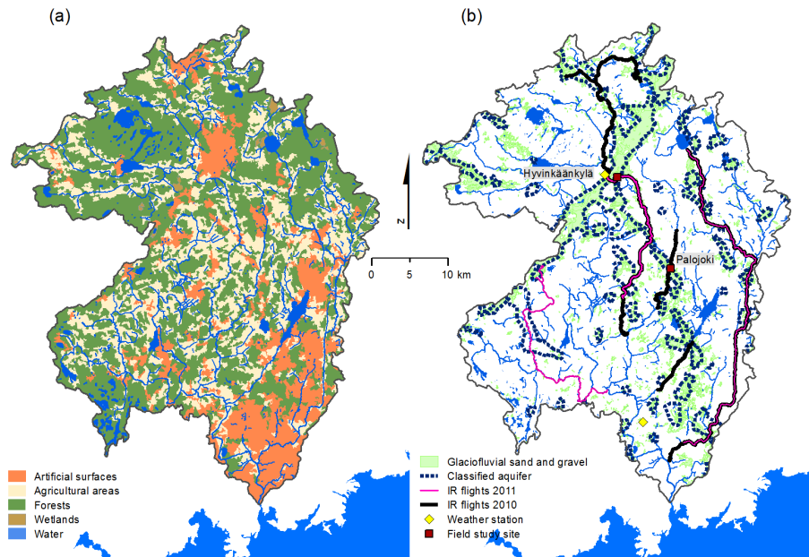
Figure 2. (a) Land use in the River Vantaa catchment. (b) AIR flights over the Rivers Vantaa, Herajoki, Palojoeki, Keravanjoki, Tuusulanjoki and Lepsämäenjoki in 2010 and 2011. (Corine land cover © National Land Survey of Finland 2010; Basemap Database © National Land Survey of Finland 2010; Quaternary Deposit Database © Geological Survey of Finland 2008; Groundwater Database © SYKE 2010; Watershed Database © SYKE 2010).
