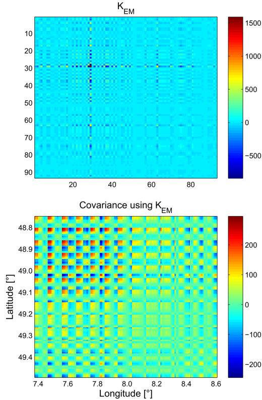
Figure 13. Estimate of the covariance matrix K using the E-M algorithm and the corresponding covariance matrix for the Wet delay map from PSI+GNSS. The wet delay observations are aggregated into maps of 7 \times 7 km 2 cells before their covariance matrices are computed.
