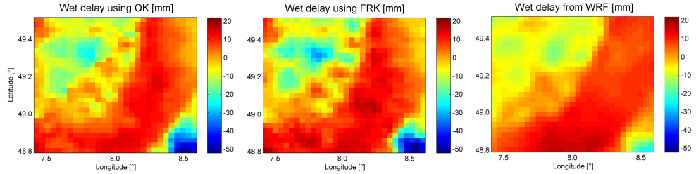
Figure 9. Wet delay prediction map using the block OK and FRK. The resolution of the grid is 3 \text{ km} \times 3 \text{ km} . A point-level wet delay map, on 23 May 2005 at 09:51 UTC, is used as input to the algorithms.
