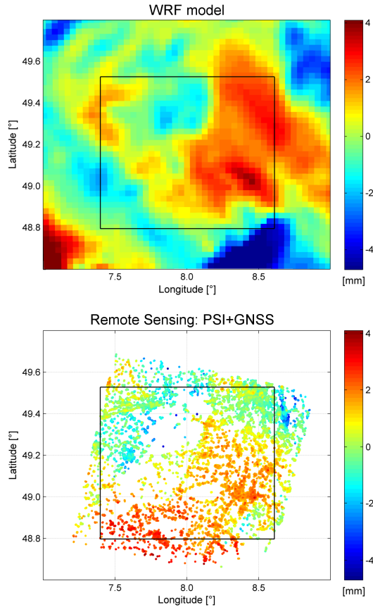
Figure 10. PWV maps from PSI+GNSS combination and WRF on 5 September 2005, with a linear trend subtracted from each map. PSI+GNSS provide point-level observations, while WRF generates block data with a block size of 3 \text{ km} \times 3 \text{ km} . The predictions will be obtained within the area indicated by the black box.
