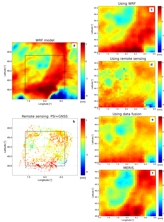
Figure 12. PWV maps from remote sensing (PSI+GNSS) and WRF model data on 27 June 2005 at 09:51 UTC as well as prediction maps obtained by data fusion and individual data sets. The output grid has a block size of 3 \text{ km} \times 3 \text{ km} over the area indicated by the black box in a and b.
