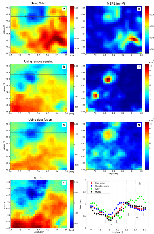
Figure 11. PWV prediction and MSPE maps obtained by data fusion of PWV estimates from PSI and GNSS and maps from WRF as well as predictions obtained by applying FRK to individual data sets. The data are available on 5 September 2005 at 09:51 UTC. The output grid has a block size of 3 \text{ km} \times 3 \text{ km} . The label A defines a region of sparse remote sensing data and the model data in region B are highly overestimated.
