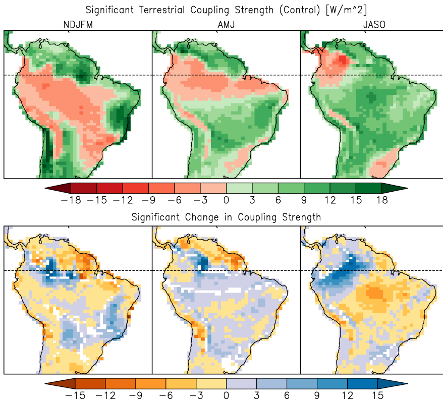
Figure 8. Terrestrial leg of coupling strength [ W/m^2 ] between soil moisture and latent heat flux for the control simulation (top-row) and change due to deforestation (bottom-row) for NDJFM, AMJ and JASO. Shading indicates significance of the correlation component at the 95% confidence level.
