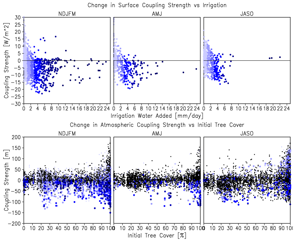
Figure 10. Top row: Change in terrestrial leg of coupling strength [ W/m^2 ] versus irrigation water added [ mm/day ] for irrigated gridboxes in NDJFM, AMJ and JASO. Bottom row: Change in atmospheric leg of coupling strength [ m ] versus initial tree cover percentage for NDJFM, AMJ and JASO. Shaded dots represent irrigated gridboxes with the shading being equivalent to the shading for irrigation water added [ mm/day ] in top row.
