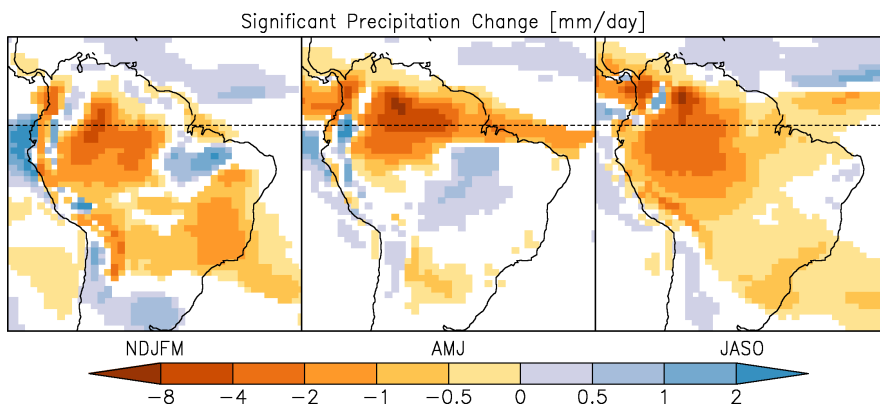
Figure 5. Change in precipitation [mm/day] for NDJFM, AMJ and JASO. Shading indicates significance at the 95% confidence level.
