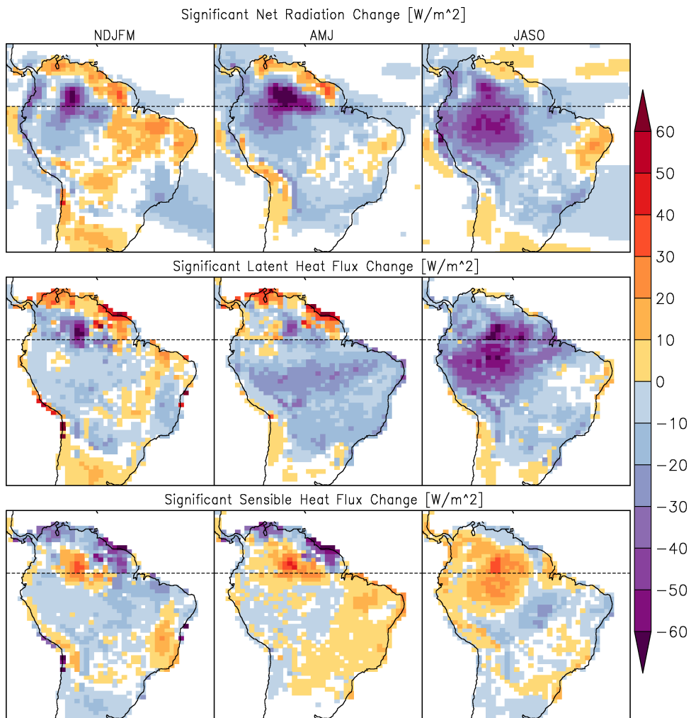
Figure 6. Changes of surface energy fluxes in NDJFM, AMJ and JASO; net radiation [ \text{W/m}^2 ] (top-row), latent heat flux [ \text{W/m}^2 ] (middle-row) and sensible heat flux [ \text{W/m}^2 ] (bottom-row). Shading indicates significance at the 95% confidence level.
