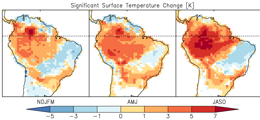
Figure 4. Change in surface temperature [K] for NDJFM, AMJ and JASO. Shading indicates significance at the 95% confidence level.
