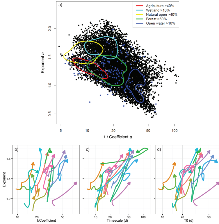
Figure 4. a) Landcover controls on Brutsaert–Nieber recession parameters a and b . The contours represent the 80 % probability region for 10 km gridcells with a dominant landcover. Black dots represent the normalized 10 km grid cells; blue dots the original catchments. b) Trends in 1/a and b for the period 1950–2000, for a representative subset of catchments. Values are computed per catchment and year, using moving and overlapping 5-year time windows and smoothed in the time domain with a LOESS smoother. Colors identify individual catchments. c) Similar, but using the time scale T (Eq. (5), using the 95th percentile of Q as Q_0 ). d) Similar, but using the time scale T_0 (Eq. (6)).
