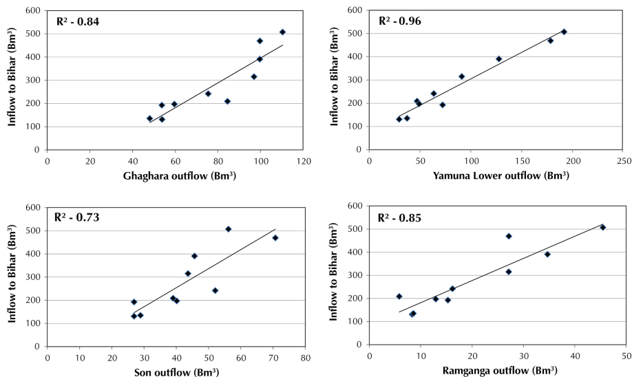
Figure 5. Relationship between outflows from upstream sub-basins and inflow to the State of Bihar.
