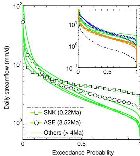
Figure 7. Flow duration curves for the catchments whose aridity index are in the range between 0.35 and 0.45. Inset of this figure illustrates flow duration curves for all study catchments. Each colored line represents data from a certain range in aridity index (key to line colors is as follows: blue: PE/P < 0.35 ; green: 0.35 < PE/P < 0.45 ; orange: 0.45 < PE/P < 0.65 and black: PE/P > 0.65 ).
