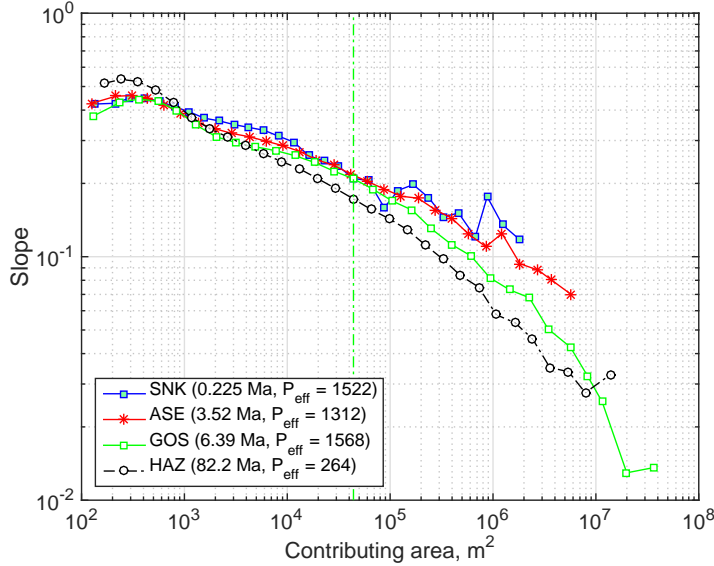
Figure 10. Mean slope area relationship for the catchments with tectonic uplift of 250 m in the Quaternary. Vertical dashed lines represent visually determined larger inflection point for GOS ( 4.4 \times 10^4 \text{ m}^2 ).
