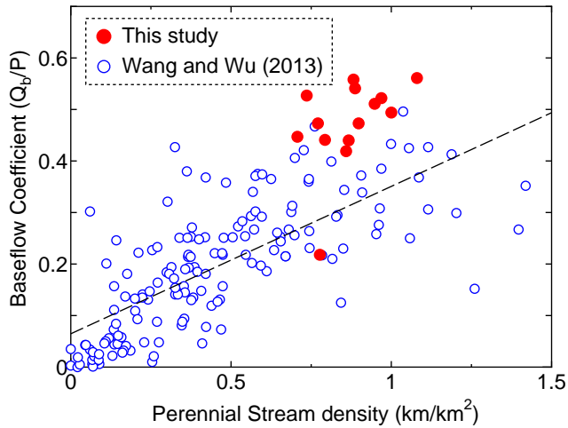
Figure 16. Perennial stream density and baseflow coefficient ( Q_b/P ). The baseflow, Q_b , in their study was estimated by using the same equation and parameter value as we used in equation (3). The correlation coefficient between them was 0.74 without the study catchments (Wang and Wu, 2013) and 0.72 for the entire dataset
