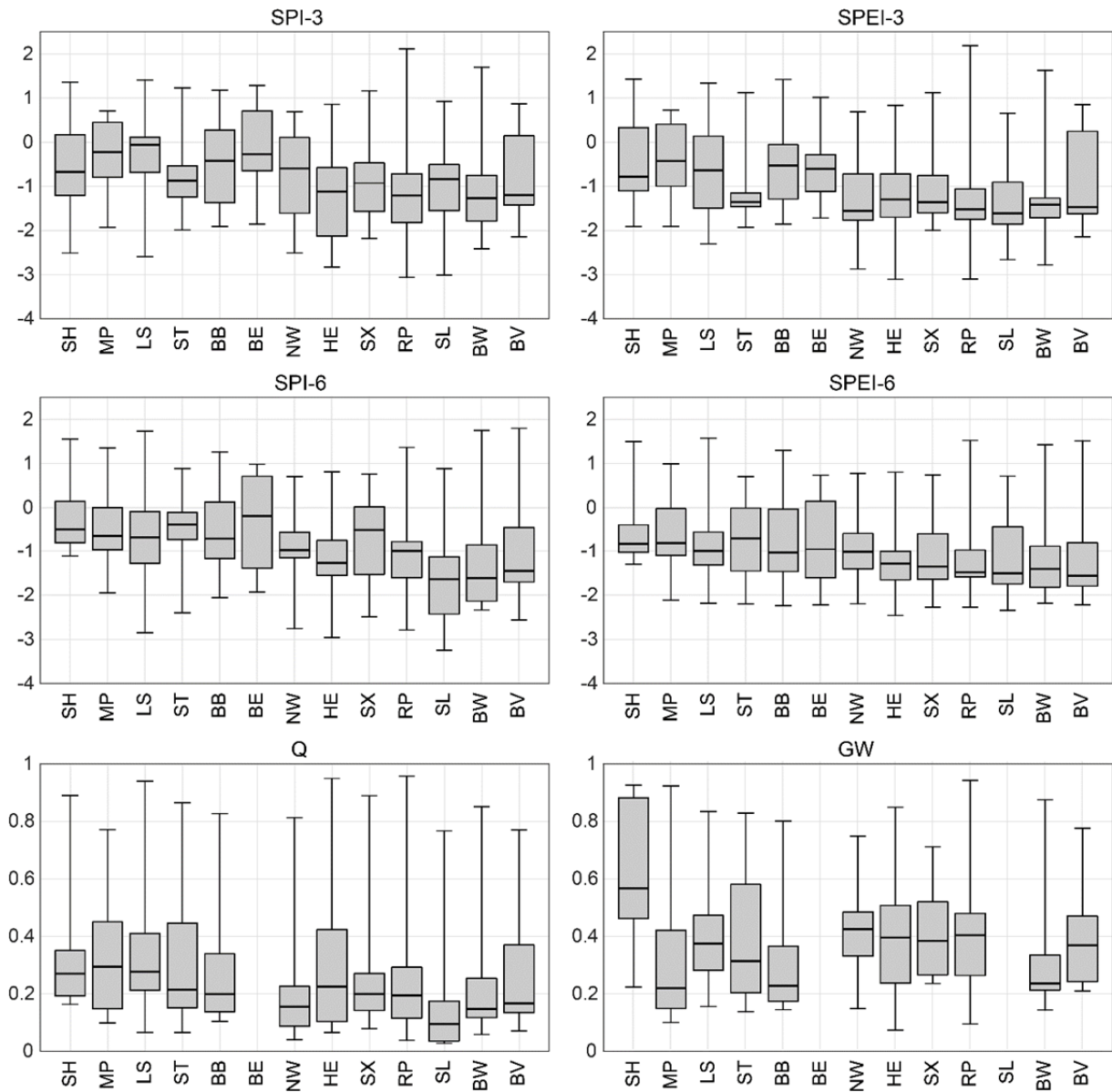
2 Figure 9: Germany: distribution of splitting values during random forest construction (i.e. 3 thresholds of selected drought indicator variables for each NUTS1 region. Boxplots as Figure 4 8.
