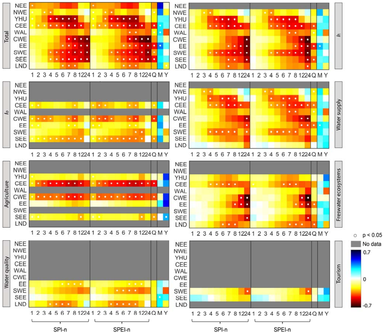
1 2 Figure 3: UK: rank correlation coefficients ( \rho ) between drought indicators and number of 3 impact occurrences for total impacts, hydrological drought impacts ( I_h ), impacts due to other 4 types of drought ( I_o ), and selected impact categories per NUTS1 region.
