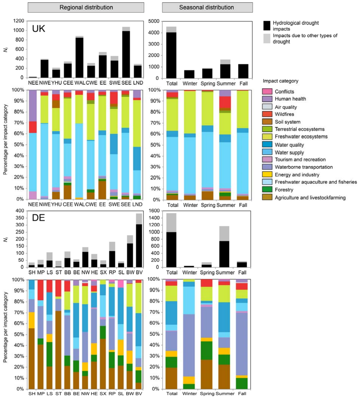
2 Figure 2: Number of impact occurrences and distribution of impacts per impact category per 3 NUTS1 region and season for the UK (top four plots) and Germany (bottom four plots).
