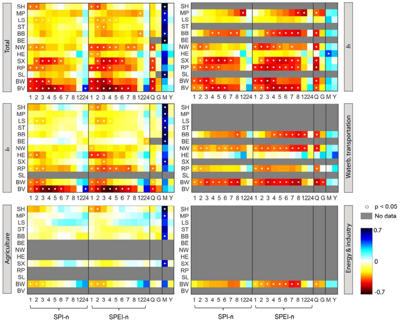
3 Figure 5: Germany: rank correlation coefficients ( \rho ) between drought indicators and number 4 of impact occurrences for total impacts, hydrological drought impacts ( I_h ), impacts due to 5 other types of drought ( I_o ), and selected impact categories per NUTS1 region. 6
