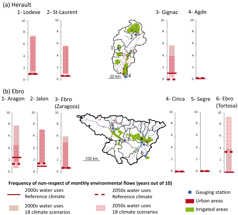
Figure 7. Frequency of years (out of ten) with monthly influenced streamflow inferior to the objective monthly environmental flow Q_{OBI} in (a) the Herault basin and (b) the Ebro basin. Frequencies are considered acceptable under two years out of 10.
