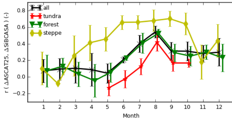
Figure 3. The seasonal variation of the spatial correlation coefficient of SiBCASA and ASCAT soil moisture for all grid cells (black \times ), tundra cells (red \star ), forest (green \Delta ) and steppe (light green \diamond ). The errorbars indicate the variation between the years 2007–2013.
