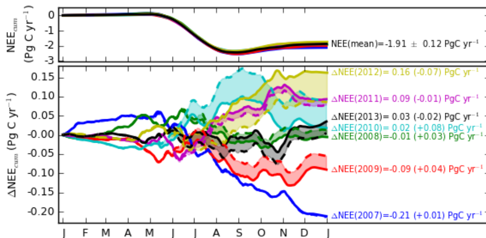
Figure 11. Top: cumulative NEE in Boreal Eurasia for the years 2007–2013 according to SiBCASA without assimilation of satellite observed soil moisture. The text describes the 7-year mean NEE and the inter-annual variation (as standard deviation). Bottom: Cumulative NEE anomaly relative to the 7-year mean. Solid lines represent the SiBCASA NEE anomaly ( \Delta\text{NEE} ) without assimilation of ASCAT soil moisture, dashed lines represent the NEE anomaly with assimilation of ASCAT soil moisture. The text behind the lines describes the NEE anomaly relative to the inter-annual mean NEE and in brackets the change caused by assimilation of ASCAT soil moisture.
