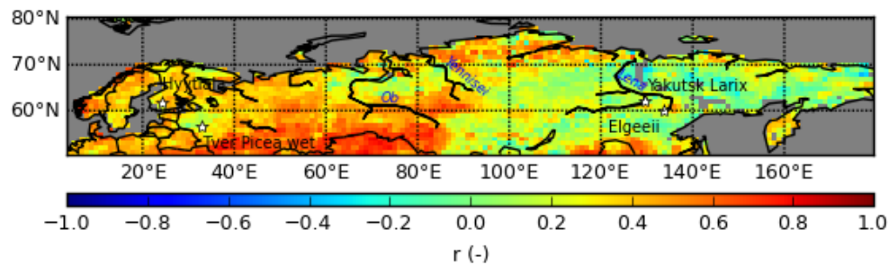
Figure 4. The temporal correlation coefficient of SiBCASA and ASCAT soil moisture for all August months in the period 2007–2013.
