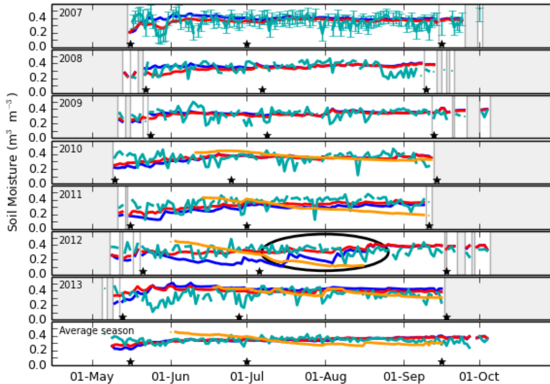
Figure 8. As Fig. 5, but for the Elgeei site.
