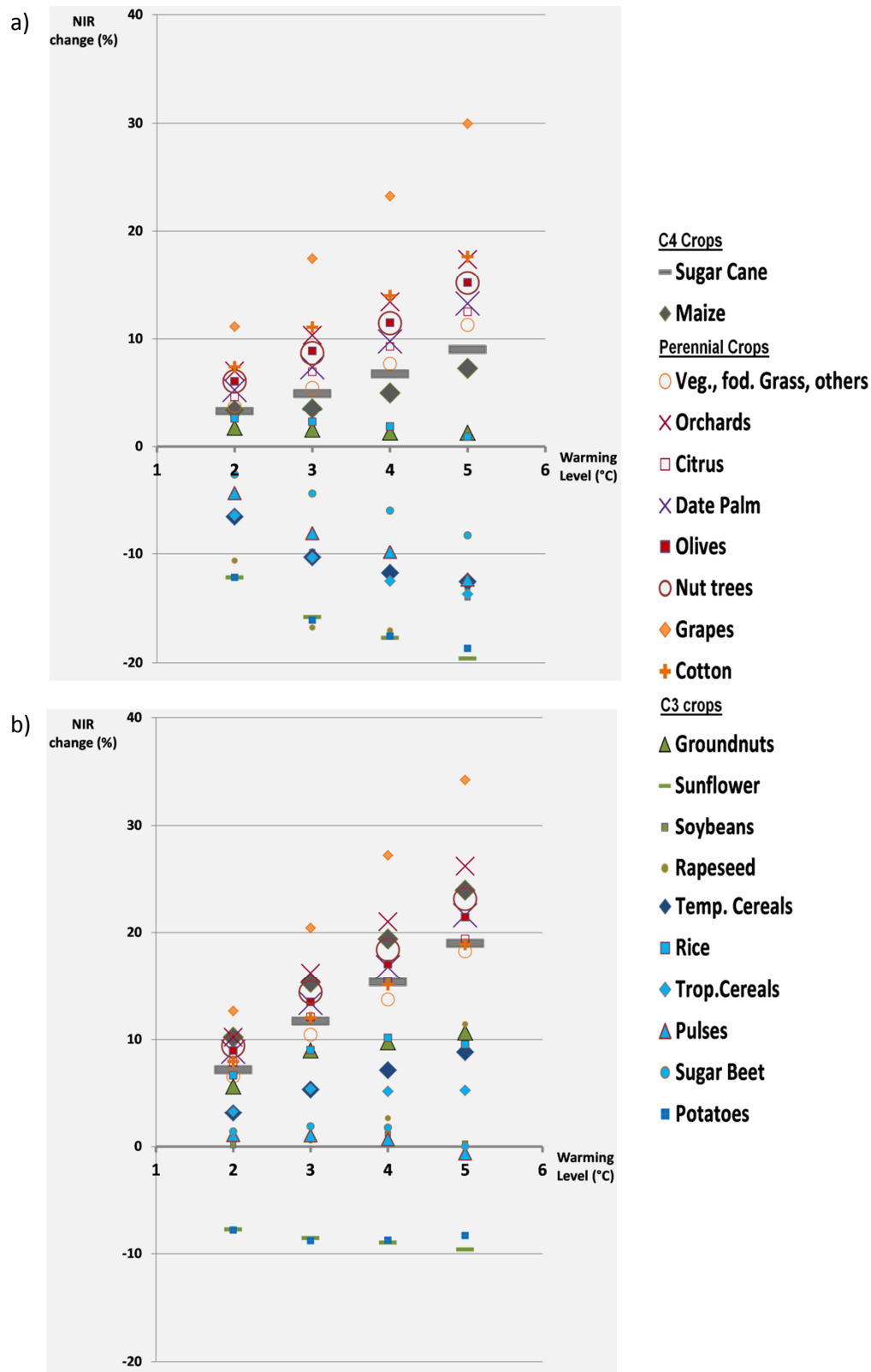
Figure 6: Change in per unit of area net irrigation water requirements NIR from 2000-2009 to 2080-2090 for different crops' classes and the DYN (a) and CONST (b) CO 2 -fertilization scenario. Negative (positive) values indicate a decrease (increase) in NIR (see Fig. S84 in supplementary material for the RED scenario).
