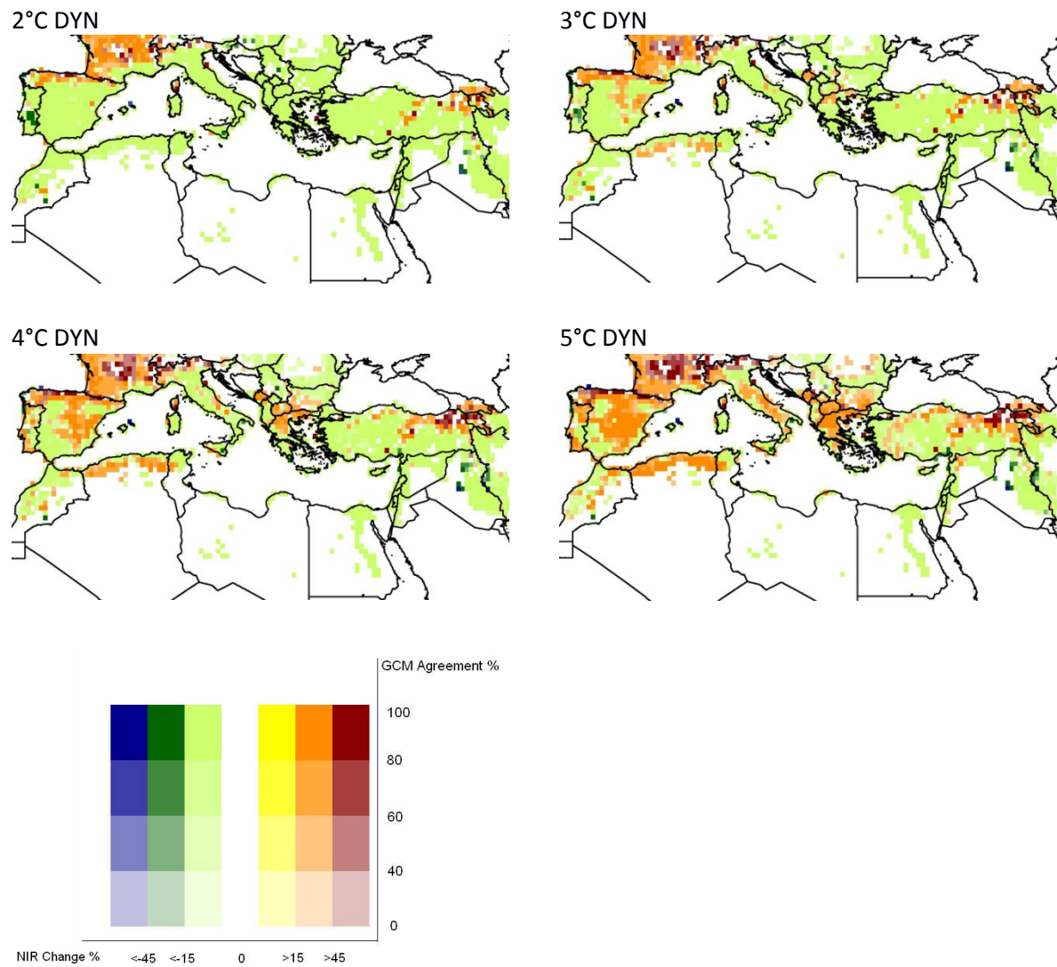
Figure S36: Change in per unit of area net irrigation water requirements NIR from 2000-2009 to 2080-2090, and GCM agreement, for different combinations of warming levels and CO 2 -fertilization scenario.
