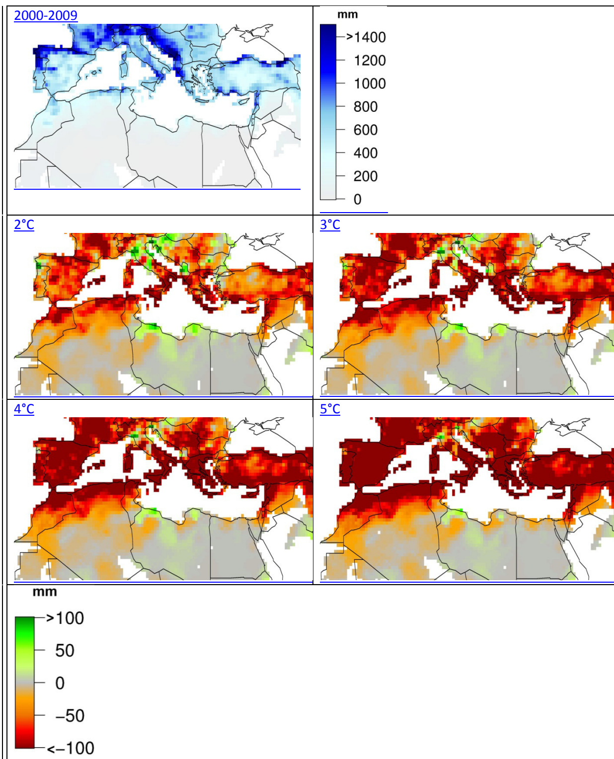
Fig. S7: Current annual precipitation as average for the period 2000-2009 (upper panel), and difference between the ensemble median of annual precipitation as average for the period 2080-2090 for 2, 3, 4 and 5 °C global warming and current annual precipitation. Negative (positive) values indicate a decrease (increase) in annual precipitation.
