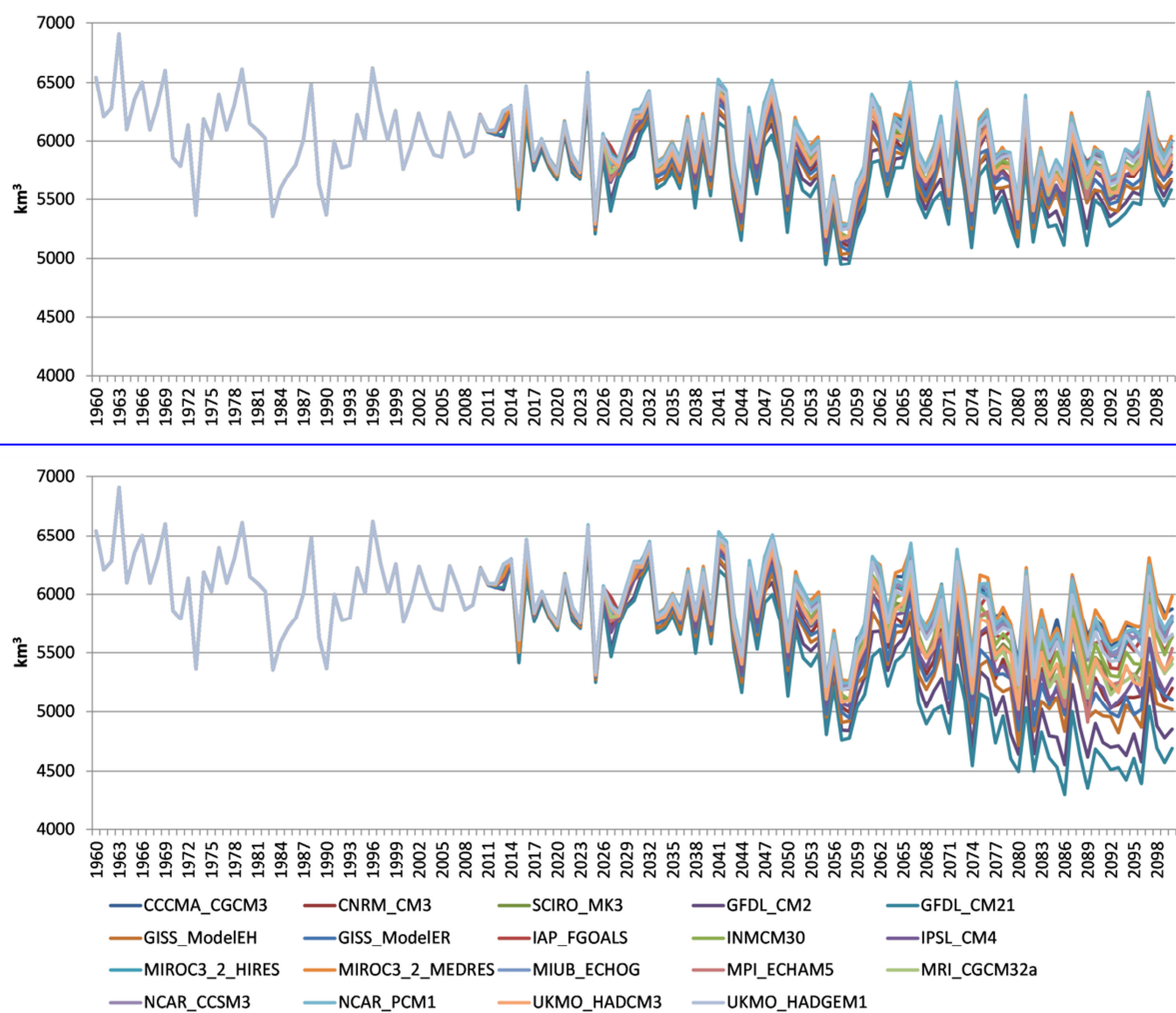
Figure S4: Time series of annual precipitation for 2°C global warming (upper panel) and 5°C global warming (lower panel) over the Mediterranean region. From 2010 to 2100 the values displayed correspond to 19 global climate models.
