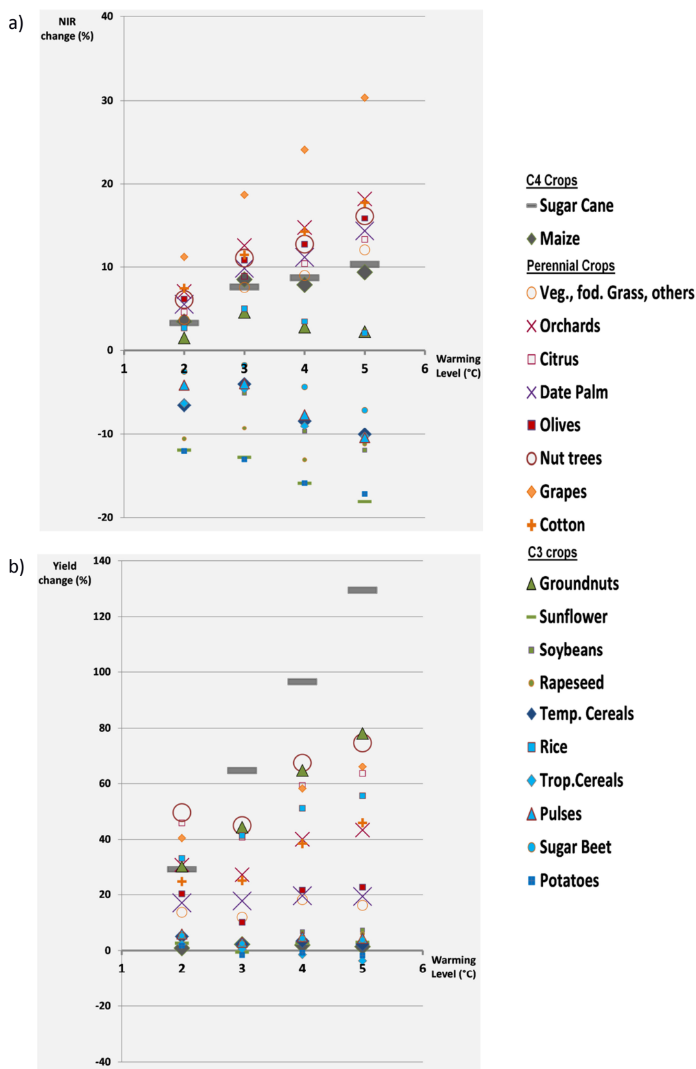
1 Figure S84: Change in net irrigation water requirements (a) and yields (b) from 2000-2009 to 2080- 2 2090 for different crops' classes and the RED CO 2 -fertilization scenario. See Fig. 6 and Fig. 7 for 3 additional scenarios.
