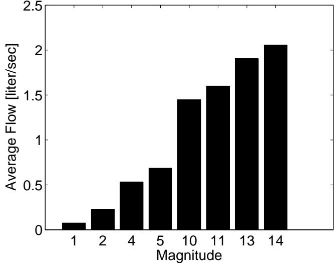
Figure 8. Average flows at different locations along the Mandelbrot-Viscek tree.
