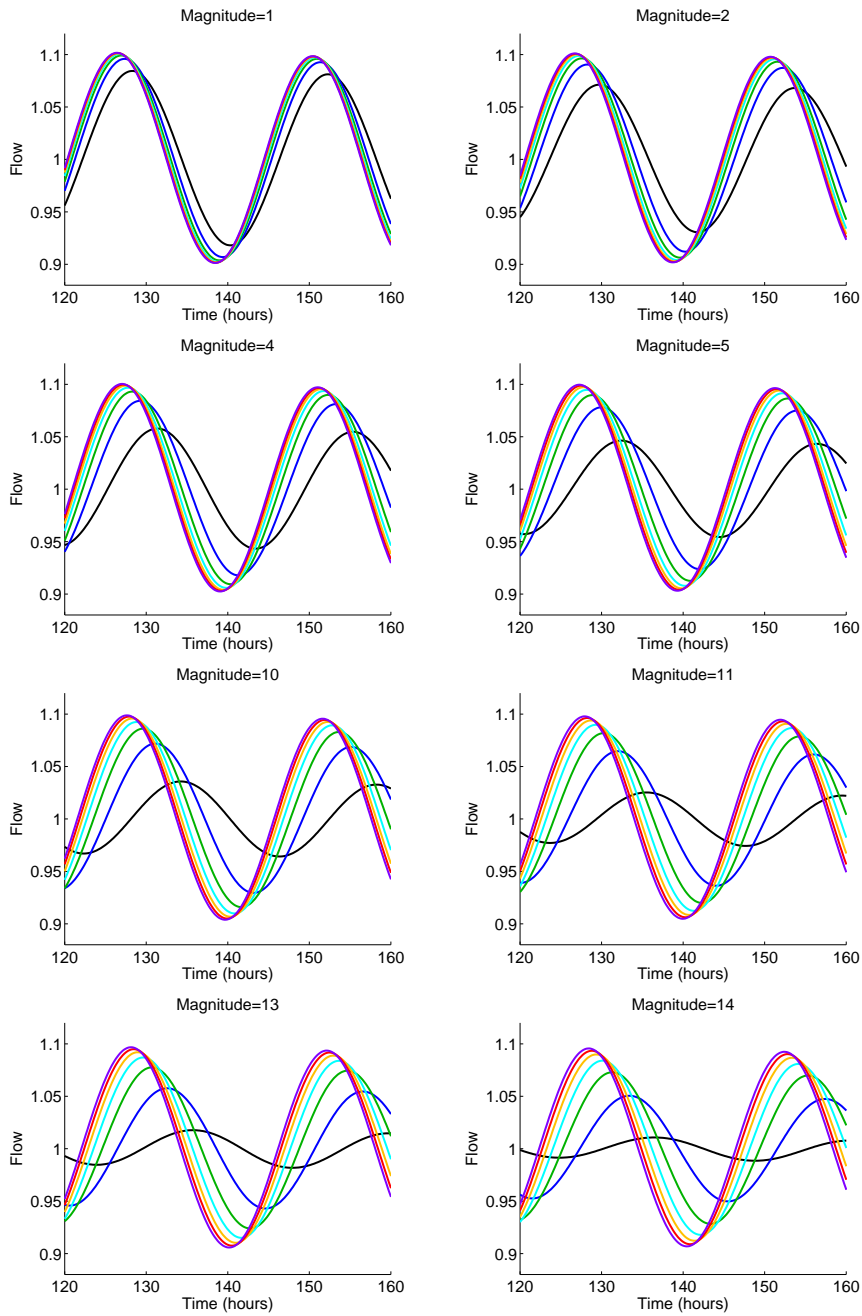
Figure 7. Flows at the outlet of each magnitude link using different k in each river simulation. The k values (with units of [\text{hr}^{-1}] ) are [0.38, 0.7, 1.02, 1.34, 1.66, 1.98, and 2.30] and are colored [black, blue, green, cyan, orange, red, and purple], respectively. The flows are normalized about the average flow.
