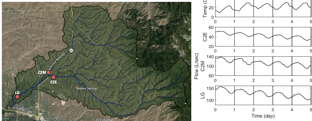
Figure 1. The left panel shows the Dry Creek watershed in Idaho. The right panel shows temperature (top), streamflow at gauge C2E near the center of the watershed (second), streamflow at gauge C2M (third), and streamflow at the outlet of the watershed (bottom). To demonstrate the delay in phases, a vertical line at the beginning of each day is included in each graph.
