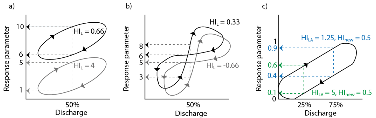
Figure 1: Plots showing a) impact of storm initial concentration, b) storm initial discharge on the value of the calculated HI when the mid-point in discharge and raw data is used and c) an idealised and normalised storm illustrating the impact of measuring different quantiles of flow on the HI calculated. Where HI_L and HI_{LA} are the original and adapted Lawler et al. (2006) methods, respectively and HI_{new} , the proposed new method. Colours represent different discharge intervals measured.
