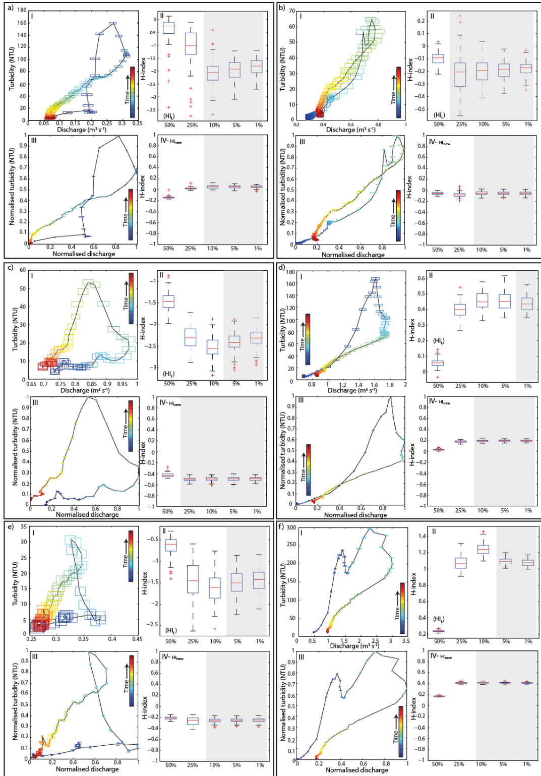
Figure 2: Plots showing six storms with varying loop shapes and sizes (a-f), where (I) is the hysteresis loop using the raw data, (II) is the distribution of HI values using the original and adapted Lawler et al. (2006) methods ( HI_L/HI_{LA} ) using varying percentiles of flow, (III) is the hysteresis loop plotted using normalised data, and (IV) is the distribution of HI values using the new method ( HI_{new} ) using varying percentiles of flow. The grey areas show the distributions which are not statistically different from each other. In panels I and III, the black line represents the median and the boxes represent the 5 th -95 th percentiles of the uncertainty range.
