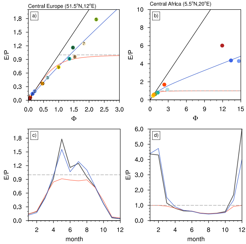
Figure 9. Data cloud of monthly climatologies within the Budyko space for a gridpoints in a) central Europe (51.5°N, 12°E) and b) central Africa (5.5°N, 20°). The black solid line denotes the demand limit, the dashed line denotes the original supply limit. The blue line depicts the obtained curve using the modified formulation of Fu's equation, whereas the red line shows the original Fu curve. Numbers within the dots denote the particular month of the year. c), d) Observed (grey) and computed mean seasonal cycles at both gridpoints. The blue line depicts the obtained seasonal cycle using the modified formulation of Fu's equation, whereas the red line shows the seasonal cycle obtained using Fu's equation. Please note that axes are different in each plot.
