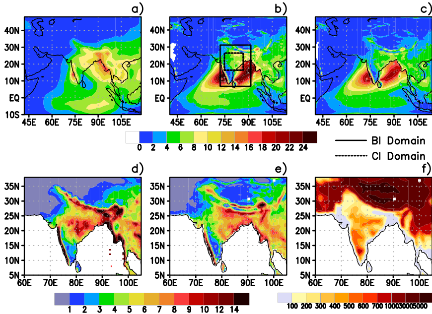
Figure 4. (a) Seasonal (JJAS) averaged rainfall from GPCP (in \text{mm day}^{-1} , 1982–2008). (b) Seasonal averaged rainfall (in \text{mm day}^{-1} ) in PLC experiment with RegCM4 (1982–2008). (c) Seasonal averaged rainfall in PLCS experiment (in \text{mm day}^{-1} , 1982–2008). (d) Seasonal averaged rainfall based on APHRODITE data (in \text{mm day}^{-1} , 1982–2007). (e) Seasonal averaged rainfall only over land in PLC experiment (in \text{mm day}^{-1} ). (f) Representation of orography in RegCM4. Units are in m.
