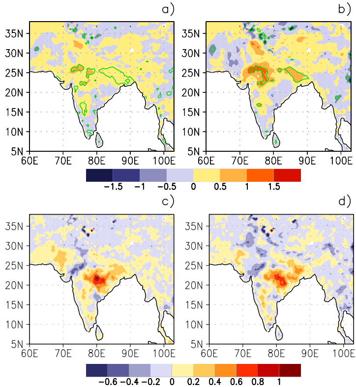
Figure 9. Difference (PLC-HLC) in daily variance of 2 m air temperature in JJAS (in °C 2 , 1982–2008) for (a) daily mean, and (b) daily maximum temperature. Green contour shows significance at 90% confidence level. Difference (PLC-HLC) in the 90th percentile of daily 2 m air temperature in JJAS (in °C, 1982–2008), for (c) daily mean and (d) daily maximum temperature.
