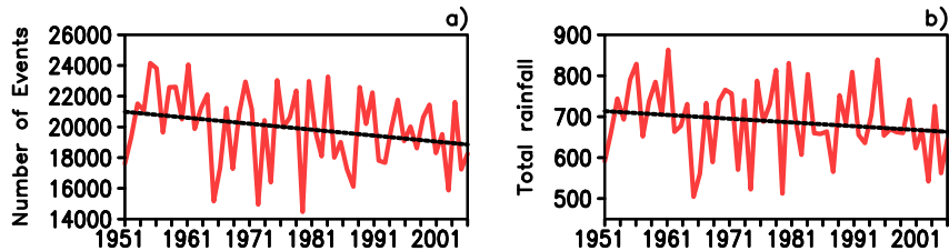
Figure 2. Time series of number of observed moderate rainfall events over CI and total rainfall in JJAS (in mm; 1951–2007) from APHRODITE rainfall data. (a) Moderate rainfall events and (b) total amount of rainfall in moderate category. Black dotted line represents the linear trend.
