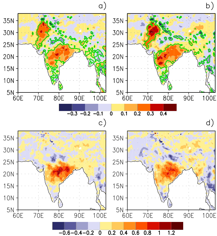
Figure 11. Difference (PLCS-HLCS) in seasonal (JJAS) averaged 2m air temperatures (in ^{\circ}\text{C} , 1982–2008) for (a) daily mean, and (b) daily maximum temperature. Green contour shows differences significant at 90% confidence level. Difference (PLCS-HLCS) in the 90th percentile of daily 2m air temperature in JJAS (in ^{\circ}\text{C} , 1982–2008), for (c) daily mean, and (d) daily maximum temperature.
