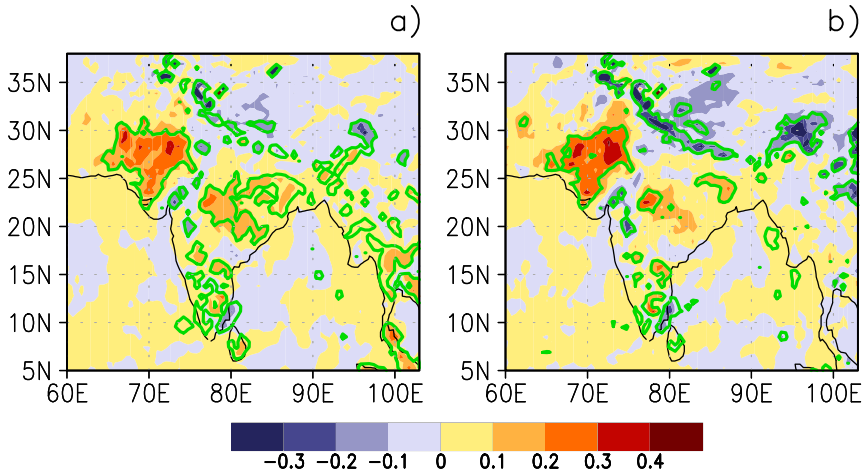
Figure 8. Difference (PLC-HLC) in JJAS averaged 2 m air temperature (in °C, 1982–2008), for (a) daily mean, and (b) daily maximum temperature. Green contour shows significance at 90% confidence levels.
