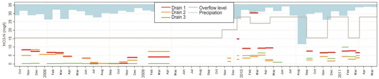
3 Figure 7: Results of the SorbiCell average NO 3 -N concentration measurements for the individual 4 drains. 5
