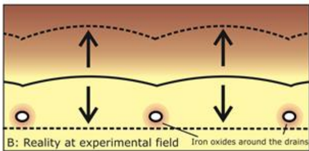
Figure 9: Comparison of (A) the common drainage concept with groundwater tables at the drain elevations and a large groundwater curvature between individual drains and (B) the situation at the experimental field with groundwater tables above the drains and a small groundwater curvature between the drains.
