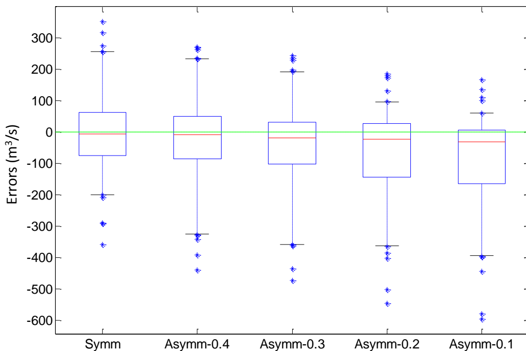
Figure 4. Parallel box-plots of the errors ( \epsilon=Q_{2,p}-Q_{2,o} ) of the 2-year floods estimates obtained by symmetric and asymmetric networks on the independent test set of catchments.
