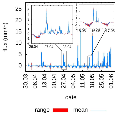
Figure 6. Variations in the calculated fluxes between the different crop lysimeters. The area in red shows the range of minimal and maximal calculations.
