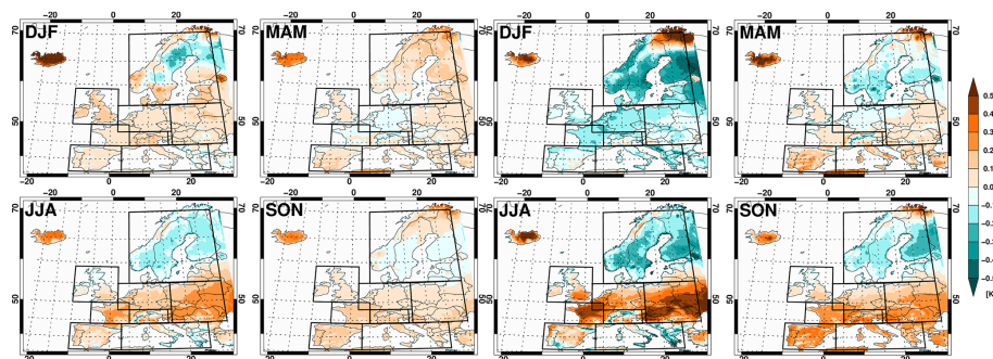
Figure 3. Differences between uncorrected and corrected (QM) multi-model standard deviation. The reference period is 1971–2000. The left panels refer to CCSs in the mid-21st century (2021–2050), the right panels to the end-21st century (2070–2099). Blue colors indicate areas where the uncorrected ensemble features a smaller standard deviation, orange colors vice-versa.
