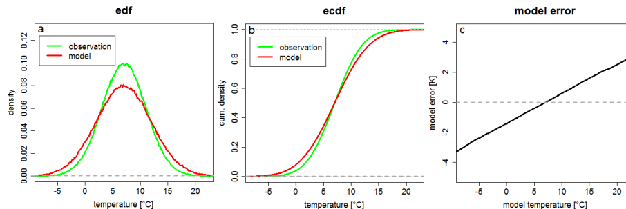
Figure 1. Intensity-dependent model errors of a model that overestimates daily temperature variability (artificial data). (a) Modeled (red, standard deviation = 5 °C) and observed (green, standard deviation = 4 °C) empirical density functions; (b) modeled (red) and observed (green) ECDFs; (c) model error at different modeled values.
