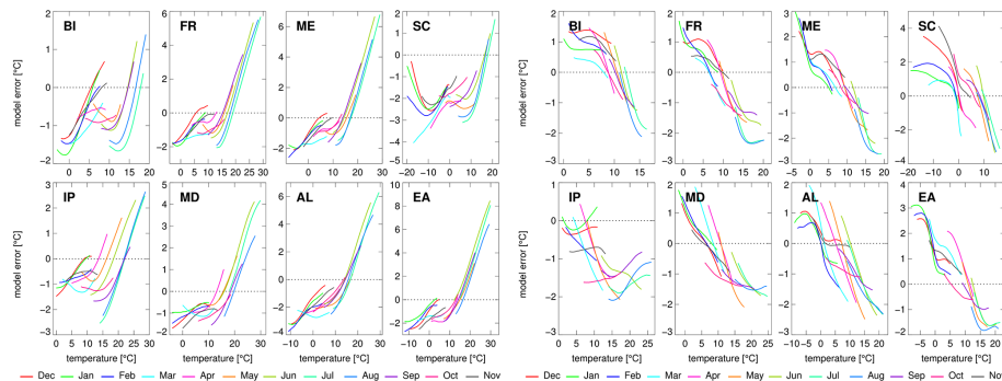
Figure 4. Temperature error characteristics (model minus observation) of the HC (left panels) and SMHI (right panels) RCMs in eight sub-regions of Europe (sub-panels) and each month of the year (colors).
