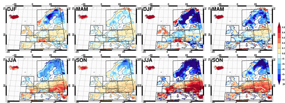
Figure 2. Differences between uncorrected and corrected (QM) multi-model mean temperature CCS. The reference period is 1971–2000. The left panels refer to CCSs in the mid-21st century (2021–2050), the right panels to the end-21st century (2070–2099). Blue colors indicate areas where the uncorrected model is colder than the corrected, red colors vice-versa.
