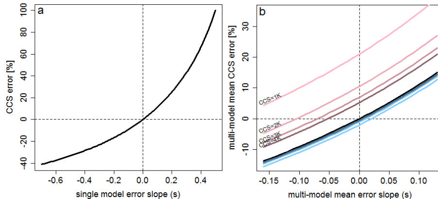
Figure 6. (a) Effect of the error slope on the single model CCS. (b) Effect of the error slope on the multi-model mean CCS. Black line: covariance term = 0 K; blue lines: covariance term = -0.02 K; pink lines: covariance term = +0.21 K. The lightest colors correspond to an error free CCS of 1 K, the darkest colors to a CCS of 4 K.
