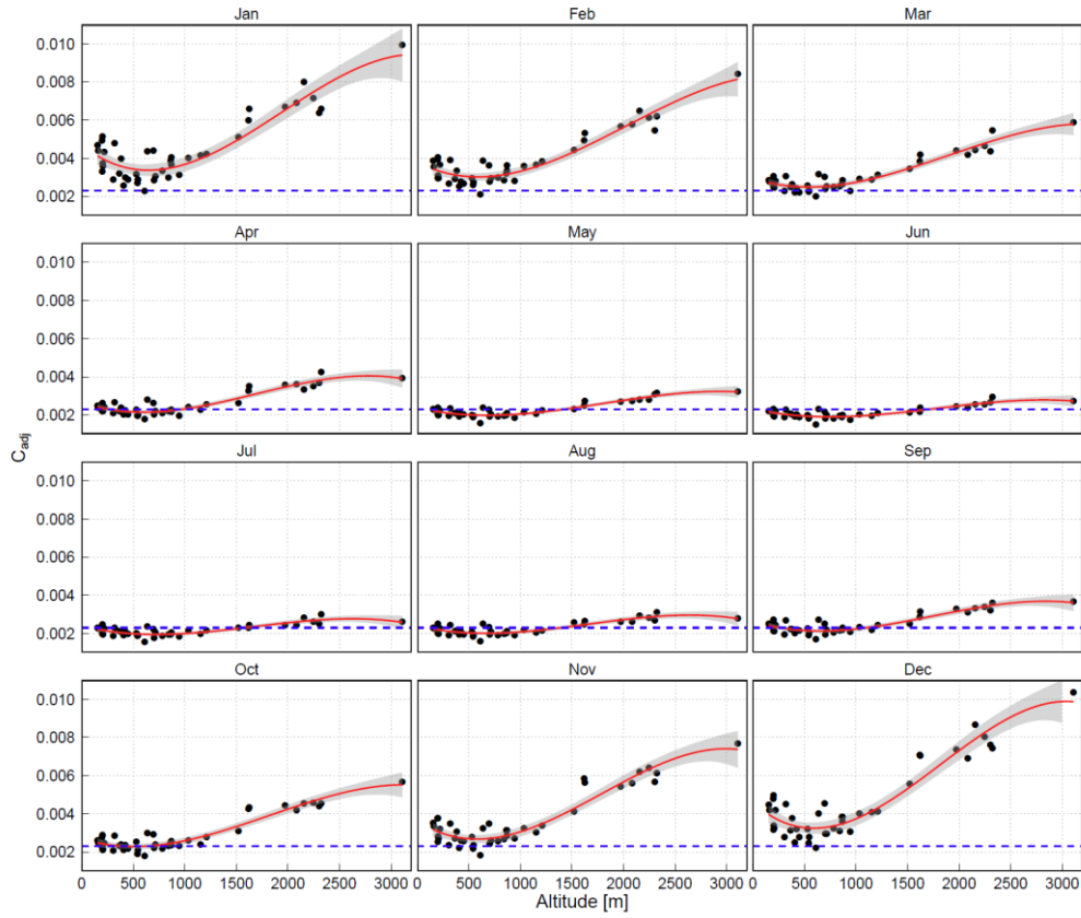
4 Figure 7. Station-wise monthly third-order polynomial fit of the Hargreaves Calibration 5 Parameter C_{adj} against altitude; the blue dotted line indicates the original C value of 0.0023.
