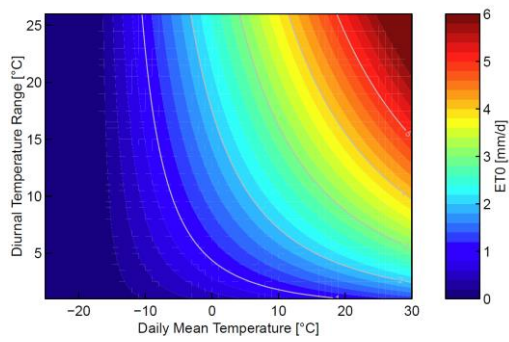
Figure 15. ET0 response to varying Daily Mean Temperature and Diurnal Temperature Range; ET0 values are calculated with 1 st of April Top of the Atmosphere Radiation and the original C value of 0.0023.
