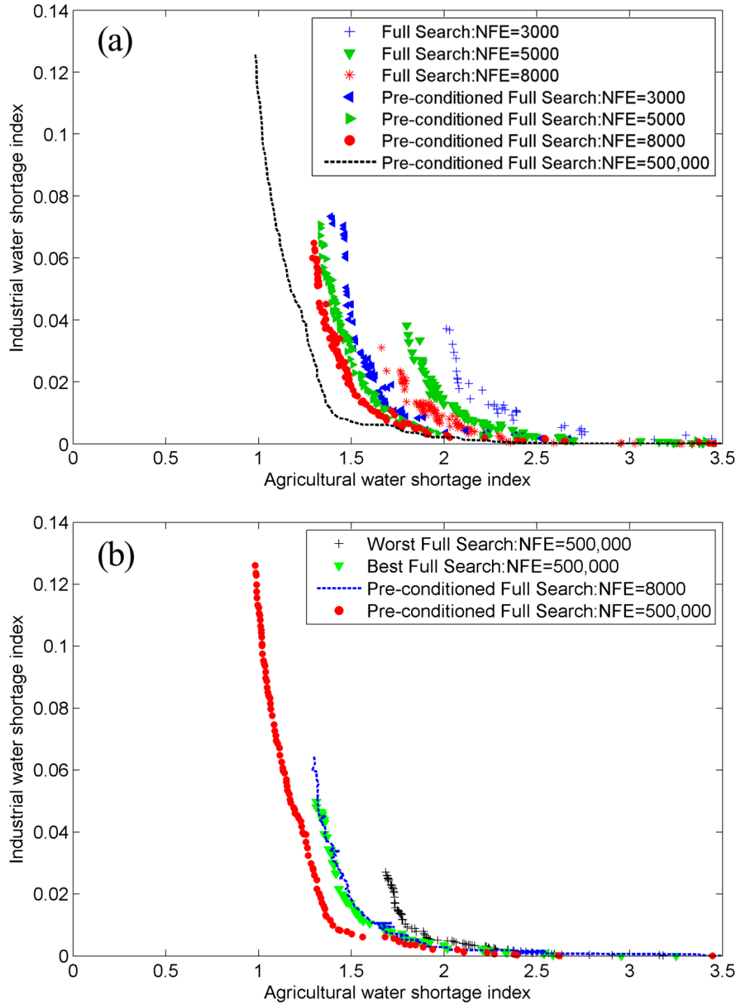
Fig. 6 Pareto fronts derived from pre-conditioned and standard full searches for the Dahufang ROS problem. (a) Sample Pareto fronts with different numbers of function evaluations for one random seed trial. (b) The best and worst Pareto fronts of ten seed trials.
