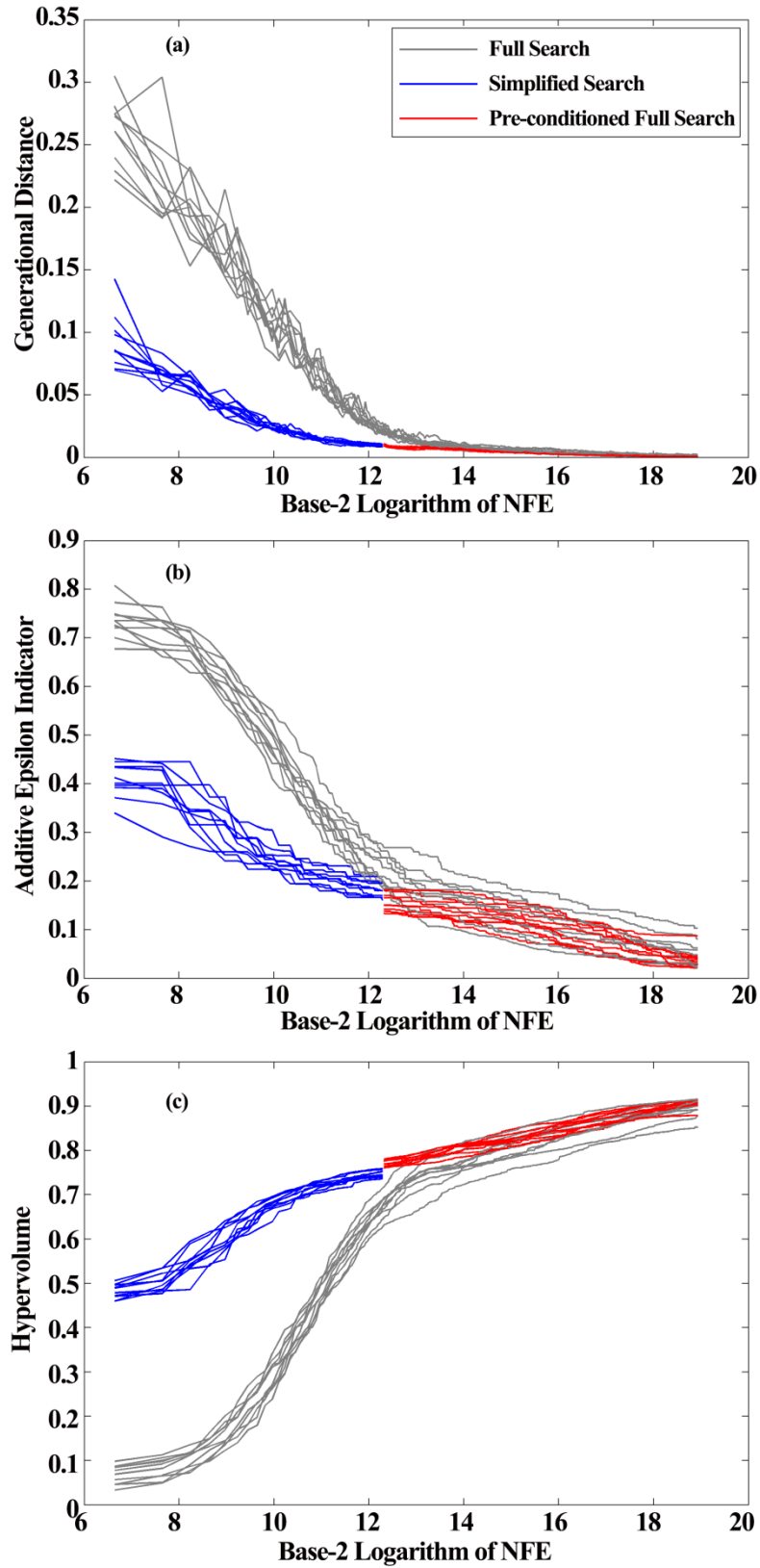
Fig. 10 Performance metrics for the inter-basin multi-reservoir water supply operation problem - (a) Generation Distance; (b) Additive Epsilon Indicator; (c) Hypervolume
