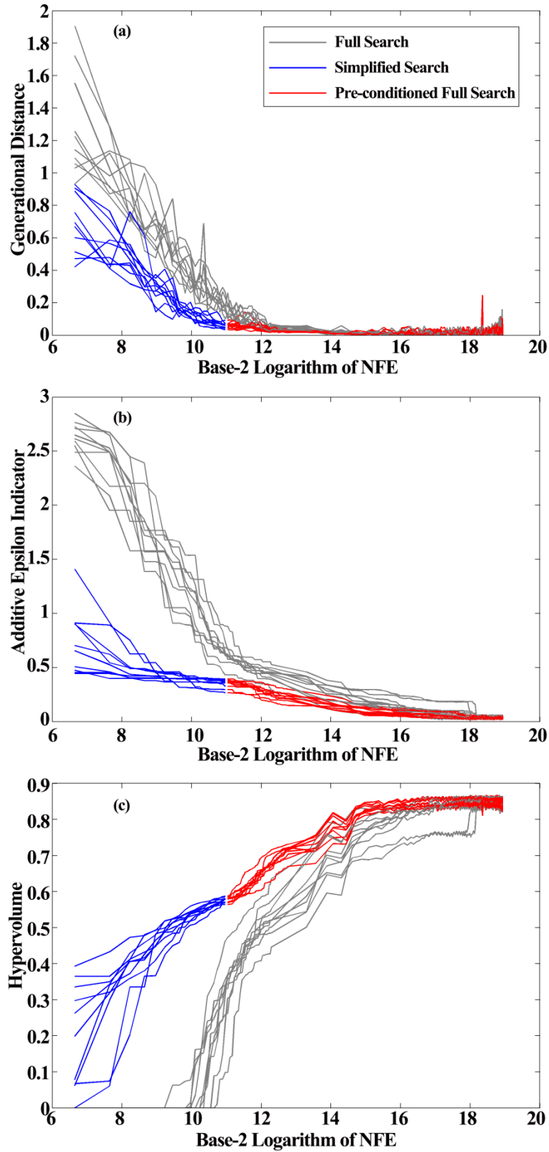
Fig. 5 Performance metrics for the Dahuofang ROS problem - (a) Generational Distance; (b) Additive Epsilon Indicator; (c) Hypervolume
