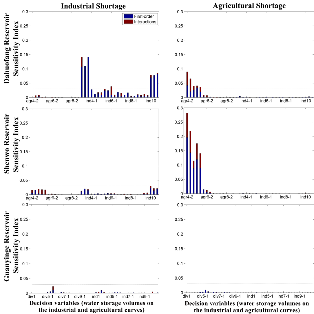
Fig. 9 First-order and total-order indices for the inter-basin multi-reservoir operation problem regarding industrial shortage index and agricultural shortage index. The x-axis labels represent decision variables (water storage volumes on the industrial, agricultural and water transferring curves)
