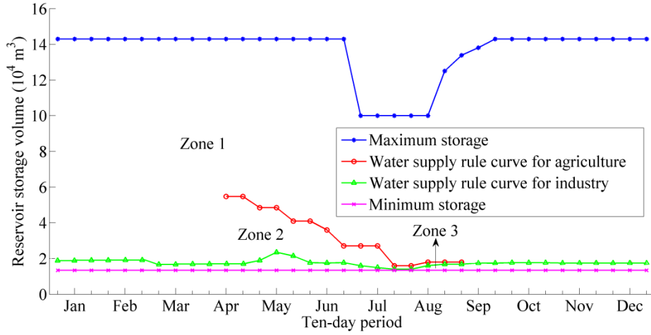
Fig. 1 Reservoir operational rule curves
