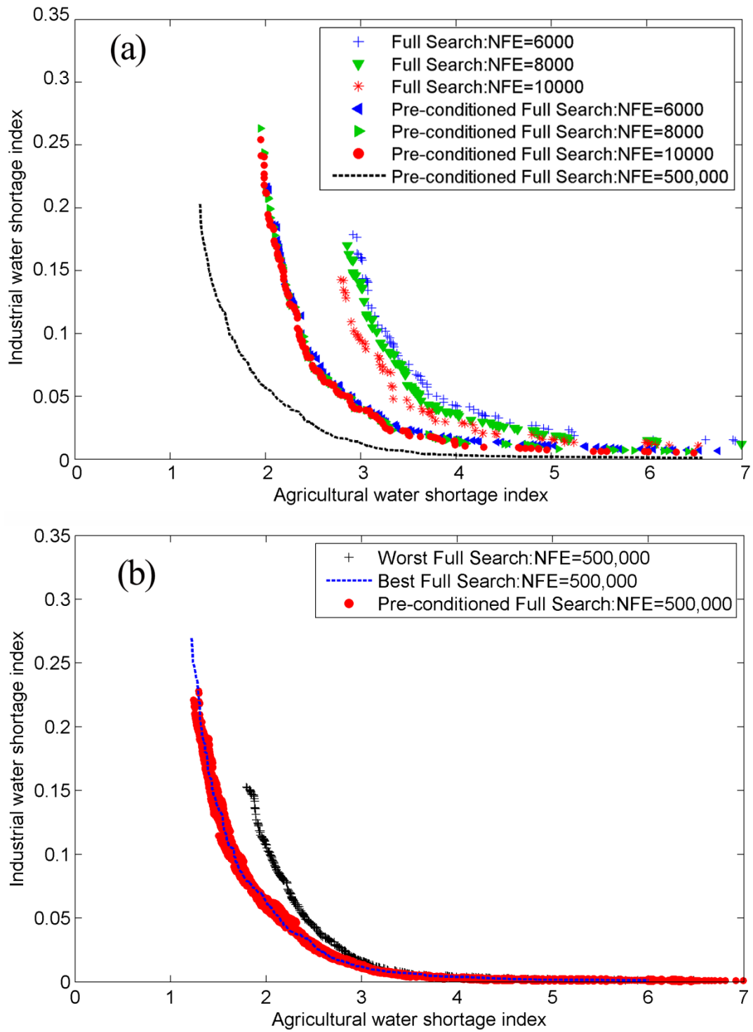
Fig. 11 Pareto fronts derived from pre-conditioned and standard full searches for the inter-basin multi-reservoir operation problem. (a) Sample Pareto fronts with different numbers of function evaluations for one random seed trial. (b) The best and worst Pareto fronts of ten seed trials.
