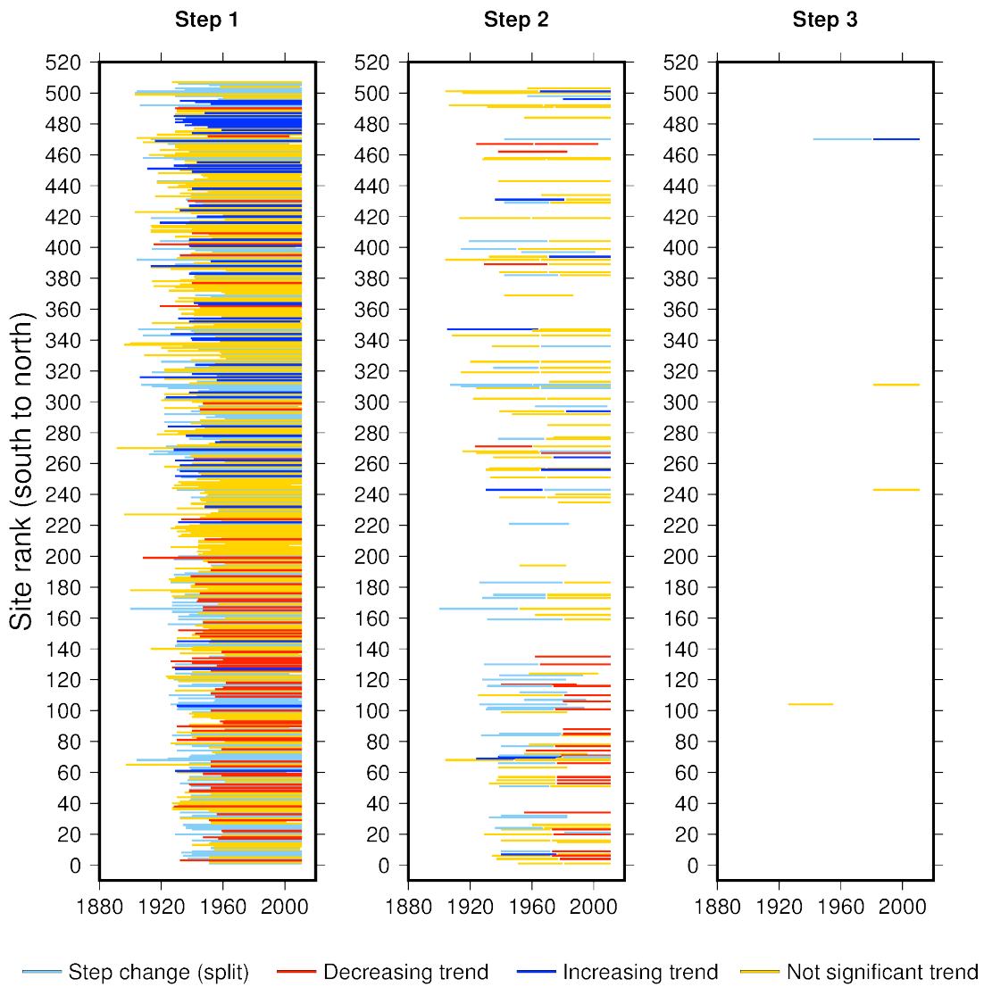
1 2 Figure 3. Range of years for each site that contain a step change, show a trend, or are 3 stationary, for each step of the decomposition algorithm.
