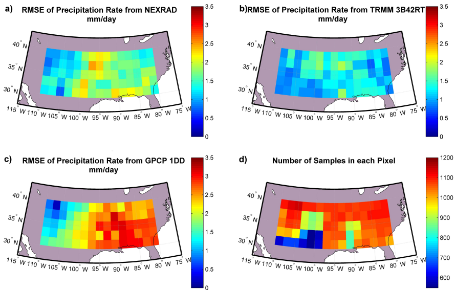
Figure 6. RMSE of the precipitation rate estimated from TC using triplets in group 2; a) NEXRAD, b) TRMM 3B42RT, c) GPCP 1DD. Panel d) shows the number of data points (biweekly measurements) in each pixel that are used for error estimation in TC analysis.
