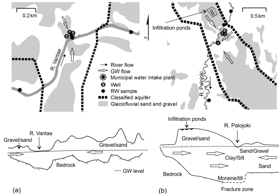
Figure 3. Schematic diagrams of the field study sites: (a) Hyvinkäänkylä field study site (bedrock elevation data from Breilin et al., 2004); and (b) River Palojoki field study sites (modified from Kortelainen and Karhu, 2006). (Basemap Database © National Land Survey of Finland 2010; Quaternary Deposit Database © Geological Survey of Finland 2008; Groundwater Database © SYKE 2010; Watershed Database © SYKE 2010).
