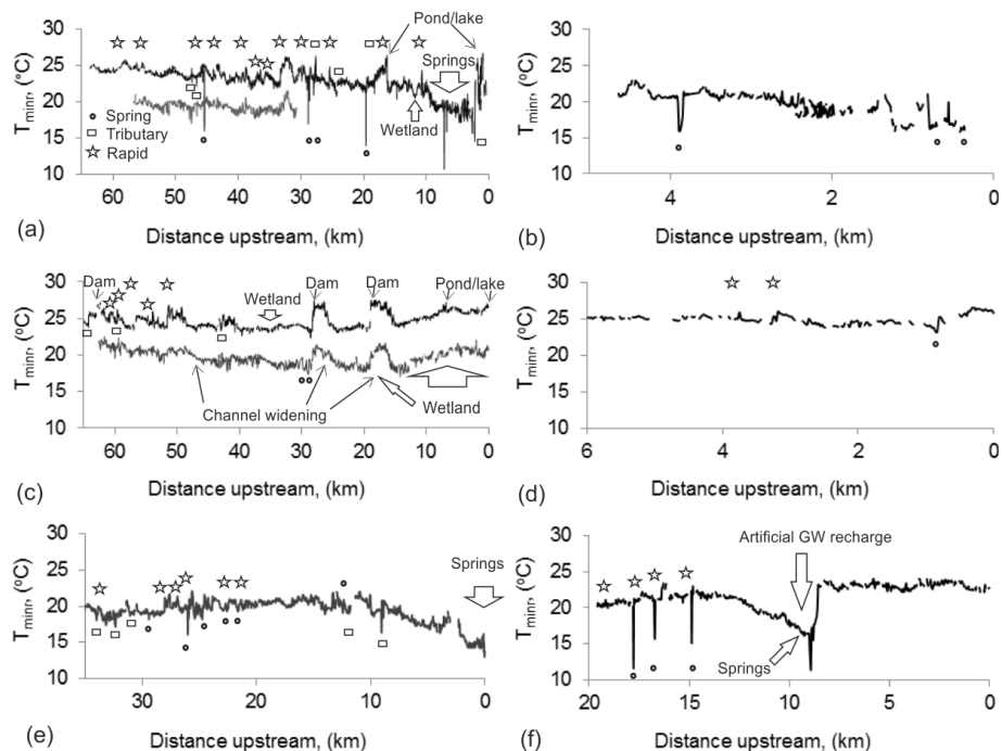
Figure 5. Longitudinal profiles of T_{\min r} of the Rivers Vantaa (a), Herajoki (b), Keravanjoki (c), Tuusulanjoki (d), Lepsämäenjoki (e) and Palojoeki (f) in 2010 and 2011. Notable tributary confluences, GWSW exchange, dams, rapids and channel morphology changes are marked in profiles.
