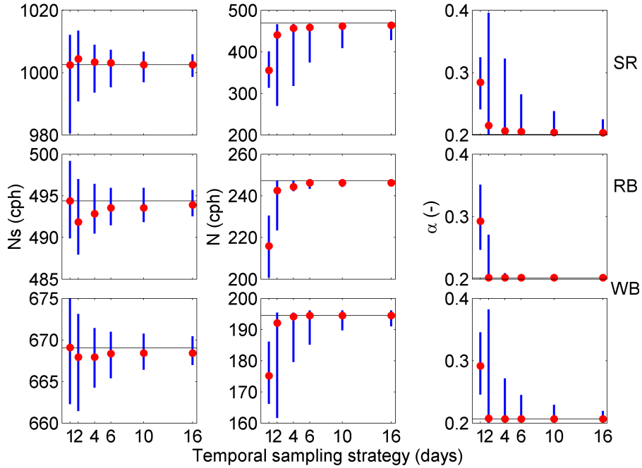
Figure 10. Parameter range distributions obtained for the best solution populations for HMF parameter N_s and COSMIC parameters N and \alpha . The parameter values of the reference strategy solutions are represented by black horizontal lines.
