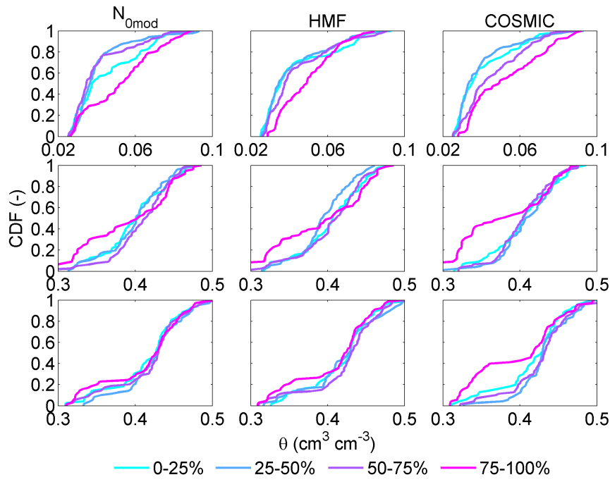
Figure 11. Cumulative Density Functions (CDF) of sub-groups from the 1DAY best solution \text{MAE}_{\text{val}} populations plotted against weighted average soil moisture content ( \theta ) (Bogena et al., 2013).
