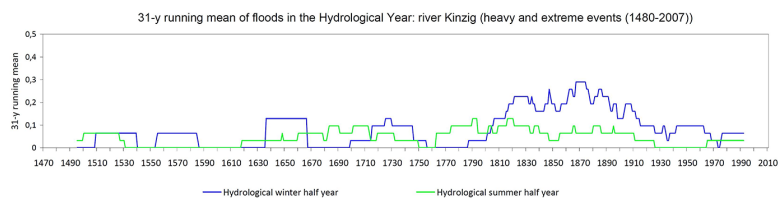
Figure 13. Floods of the river Kinzig (Baden-Wuerttemberg) in the Hydrological Summer- and Winter-Year (big and extreme events).
