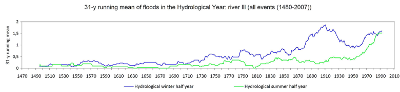
Figure 10. Floods of the river III (Alsace) in the Hydrological Summer- and Winter-Year (all events).
