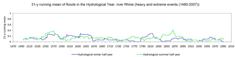
Figure 9. Floods of the river Rhine in the Hydrological Summer- and Winter-Year (big and extreme events).
