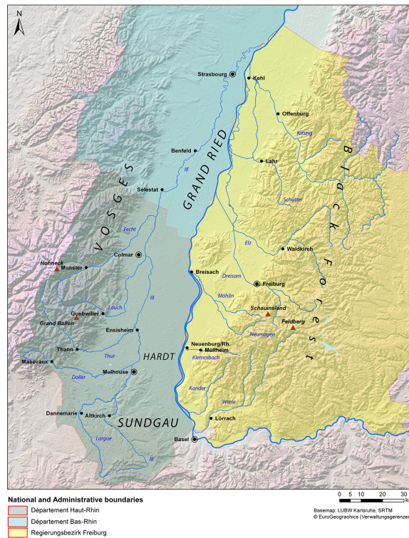
Figure 1. Study area including the researched rivers and actual administrative districts in France and Germany.
