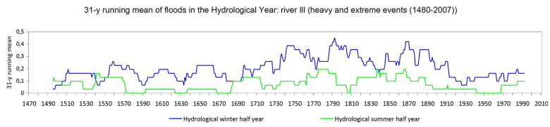
Figure 11. Floods of the river III (Alsace) in the Hydrological Summer- and Winter-Year (big and extreme events).
