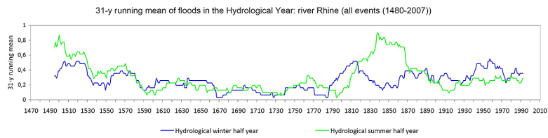
Figure 8. Floods of the river Rhine in the Hydrological Summer- and Winter-Year (all events).
