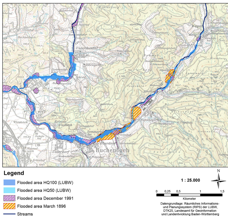
Figure 15. Comparison of flooded areas of 1896 and 1991 with modern HQ50 and HQ100 inundation areas as published by LUBW as part of the EU water directive (EU 2007).
