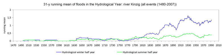
Figure 12. Floods of the river Kinzig (Baden-Wuerttemberg) in the Hydrological Summer- and Winter-Year (all events).
