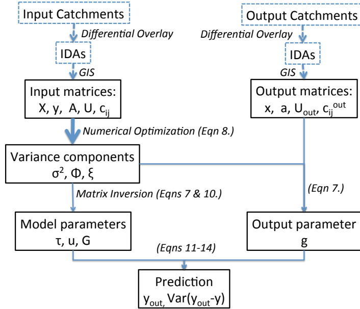
Figure 9. [ Algorithmic chart of the provided TopREML implementation. Dashed frames and arrows represent vector data and operations and the bold arrow represents the step requiring numerical optimization. The complexity of the computational tasks represented by the remaining plain arrows is driven by matrix inversion, which is of polynomial complexity. In the figure, X is a matrix of observed covariates and y a vector of outcomes measured at the available gauges, as defined in Eqn. 1; x is a vector of identical covariates observed at the prediction location. A , U and c_{ij} are matrices of relative catchment areas, network topology and inter-centroidal distances of the available gauges, as defined in Eqn 6; a , U_{out} , and c_{ij}^{out} are equivalent matrices for the prediction location. \sigma^2 , \phi and \xi are estimated variance parameters as defined in Eqn 3; \tau , u and G are the estimated fixed and random effects (Eqn 10) and variance-covariance matrix (Eqn 7); g is the estimated covariance at the prediction location (used in Eqn 11) . Finally, y_{out} and \text{Var}(y_{out} - y) are the predicted outcome and the related prediction variance. ]
