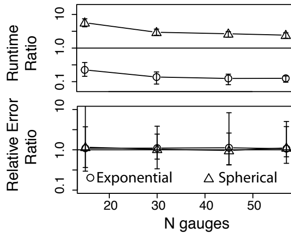
Figure 10. [ Leave-one-out cross-validation results for Austrian summer flow when resampling a subset of the training gauges. Computational performances are represented as the ratio of runtimes for TopREML against Top-Kriging. Prediction performances are represented as the ratio of relative errors. TopREML performances when using gradient based and stochastic optimization algorithms are represented as circles and triangles respectively. Points represent the median value and error bars represent 90% confidence intervals over 200 repetitions.]
