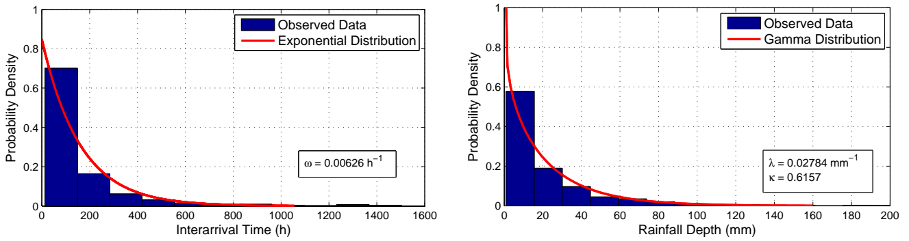
Fig. 2. Fitted distributions to interarrival times (left) and rainfall depths (right) for 25 years of data in Concepción.
