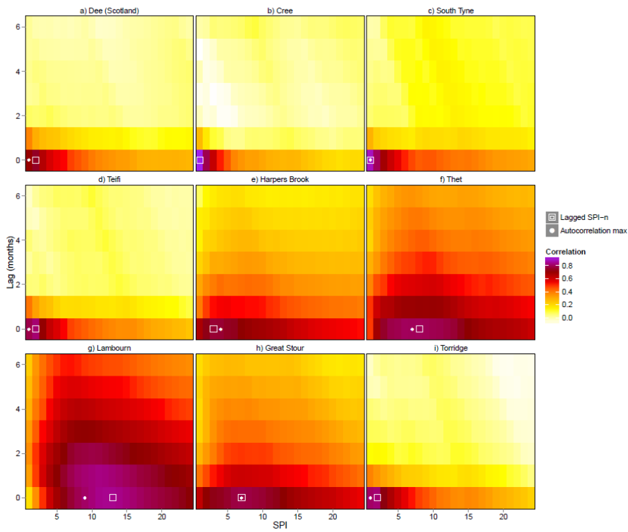
5 Figure 10. Heatmaps for case study catchments showing correlation between SSI-1 lagged by 6 0-6 months and SPI accumulation periods of 1-24 months. The lagged SPI-n is shown, as is the 7 longest n-month period for which there is significant autocorrelation in SSI-1 (autocorrelation 8 max).
