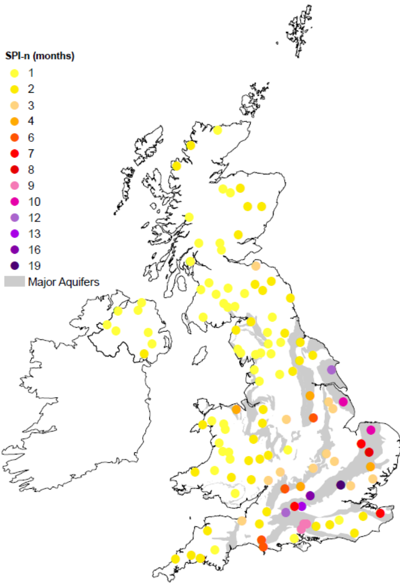
1 2 Figure 8. Map of catchments showing the SPI accumulation period most strongly correlated 3 with SSI-1 (SPI-n) and the location of major UK aquifers. 4
