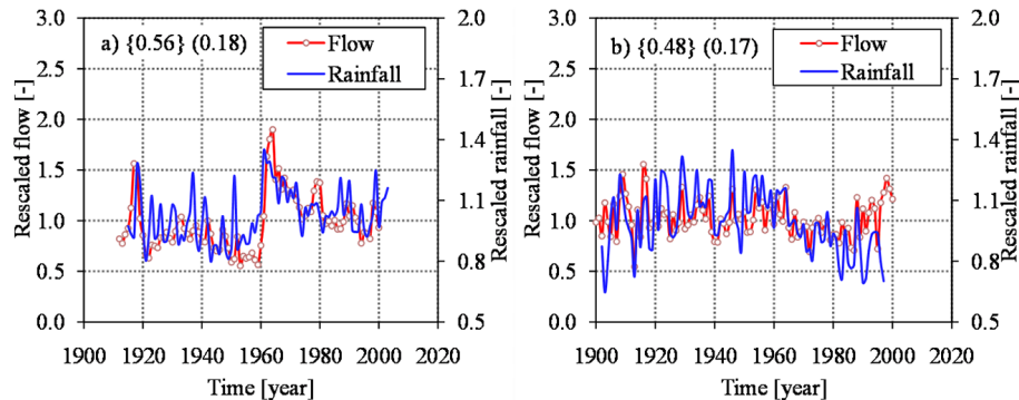
Figure 6. Variation in the region-wide annual flow and rainfall for (a) group 1, (b) group 2. The label in {} show the correlation between the annual rainfall and flow variation; and ( ) comprises the correlation critical values at 5 % significance level.
