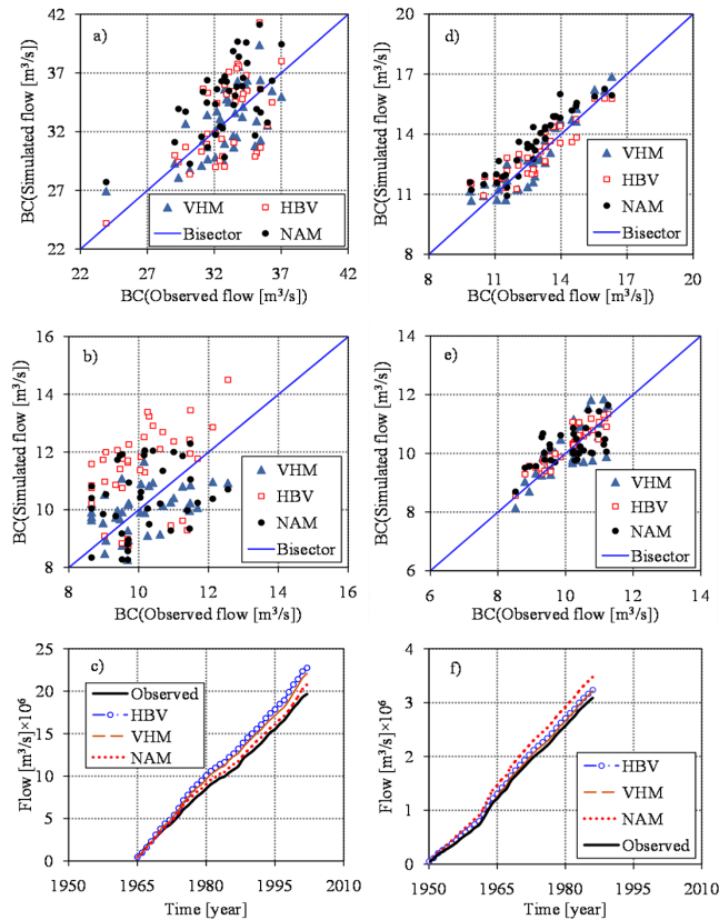
Figure 9. Evaluation of the model performance considering Box–Cox (BC) transformed (a, d) maximum flow in a year, (b, e) minimum flow in a year. Charts (c, f) are for cumulative flow, (a–c) Blue Nile catchment and (d–f) Kagera catchment.
