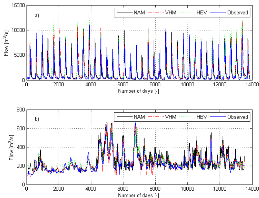
Figure 8. Simulated vs. observed daily flow for (a) Blue Nile, and (b) Kagera catchments. The calibration (validation) period cover the days 1–9131 (9132–13879) for Blue Nile, and 1–9131 (9132–13514) for Kagera.
