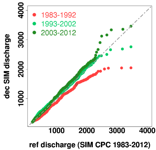
Figure 8: Quantile-Quantile plot of the distribution of daily discharge in Niamey (observed in a; simulated in b-c-d) for each decade, the reference (x axis) is the Red flood observed/simulated daily discharge between 1983 and 2012.
