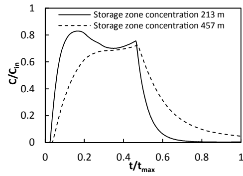
Figure 21. Simulated storage zone concentrations (test case 6)
