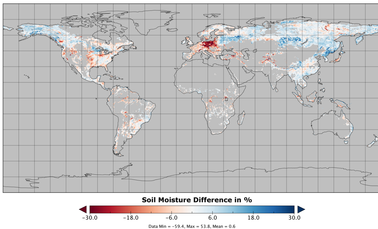
530 531 Fig. C13 Absolute differences in soil moisture for ASCAT (ASCAT NRT minus ASCAT offline) for the entire year of 532 2013 (masked according to the blending map in Fig. 4)
