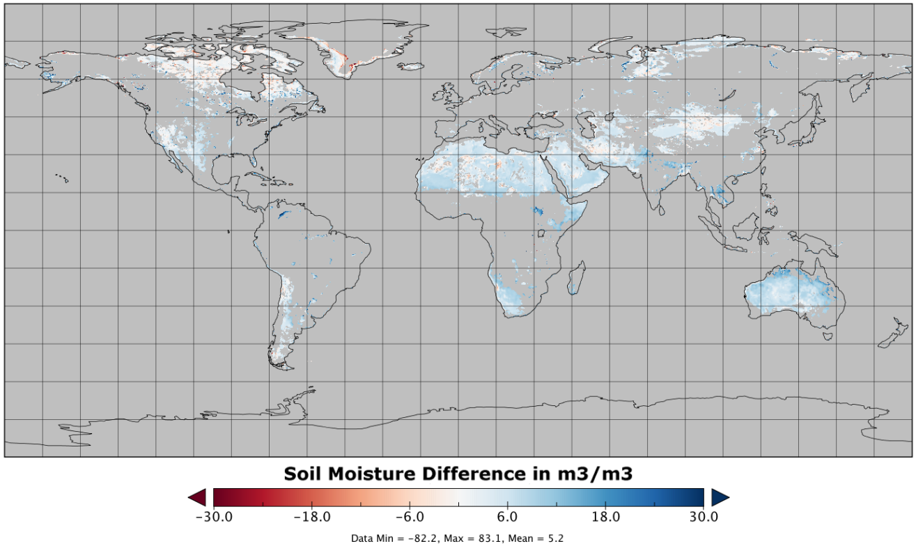
Fig. C14 Absolute differences in soil moisture for AMSR2 (AMSR2 NRT minus AMSR2 offline) for the entire year of 2013 (masked according to the blending map in Fig. 4)
