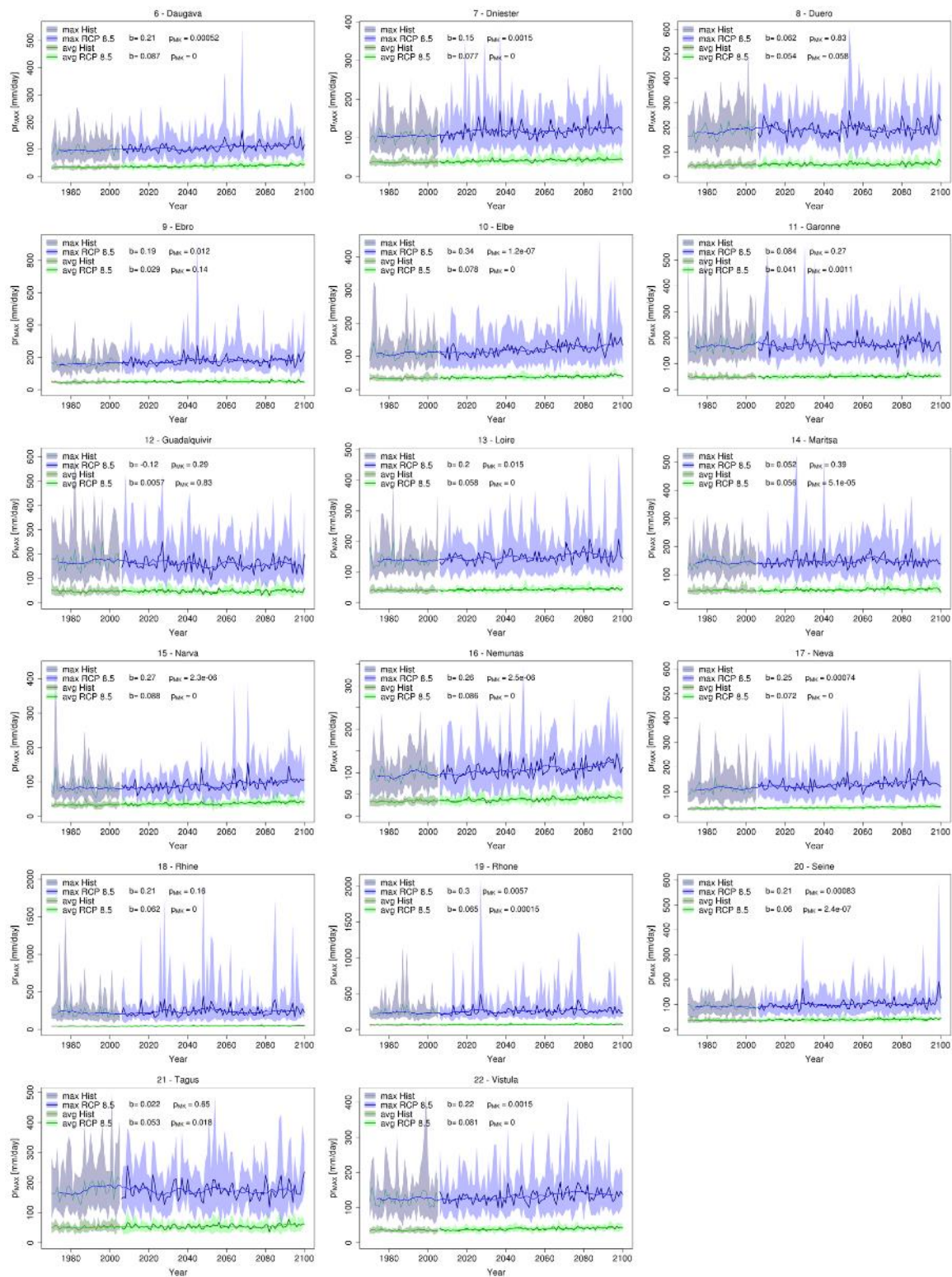
Figure S3: Annual maximum daily precipitation ( p_{MAX} ) for selected European river basins over time. Basins location is shown in Figure 1 (in yellow). Basin average (green shades) and maximum point value (blue shades) of the ensemble are shown together with the ensemble mean (thick lines) and the 10-year average (thin lines).
